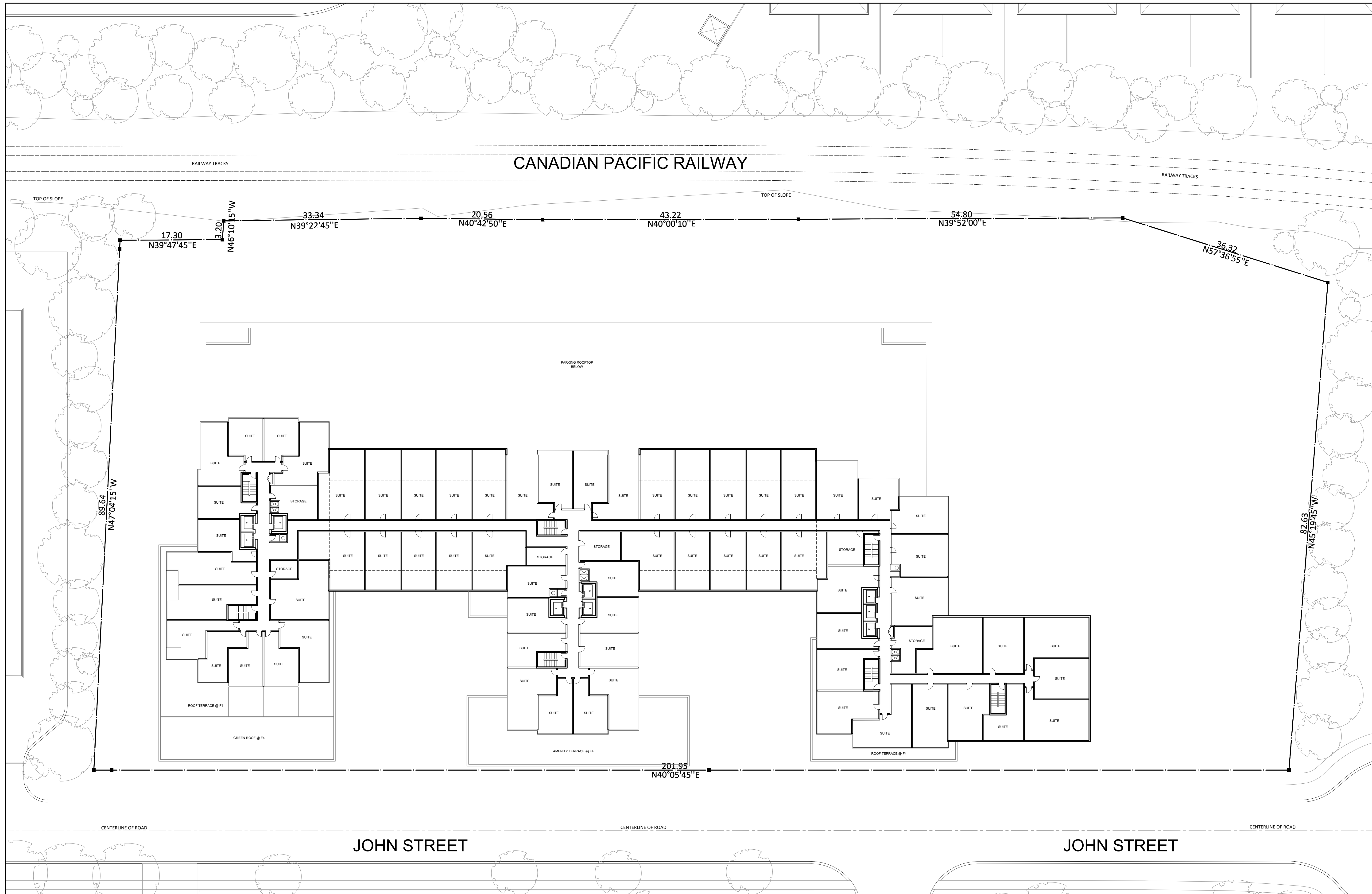
1 F8 FLOOR PLAN
