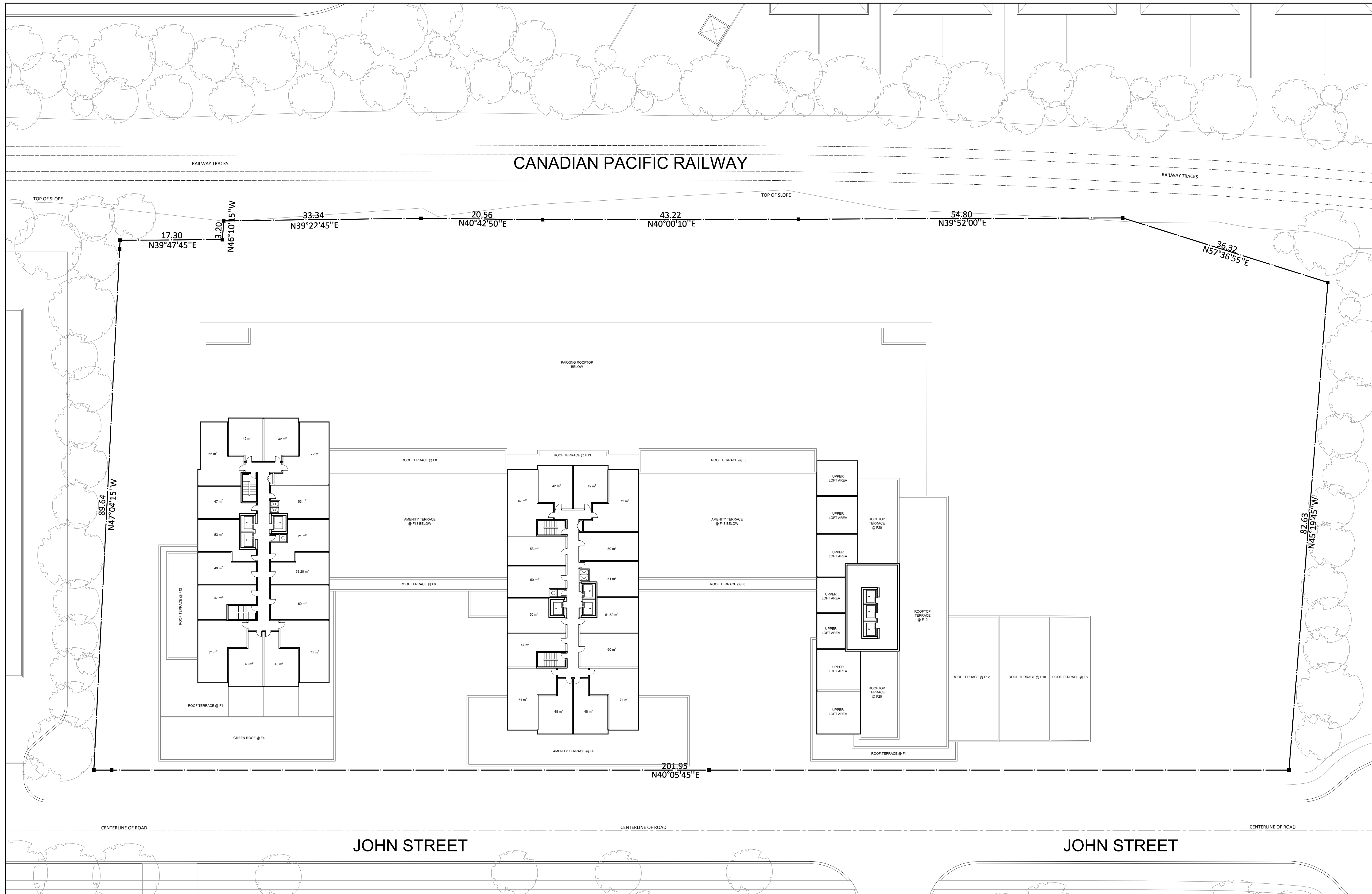
1 F20 FLOOR PLAN 1:300
