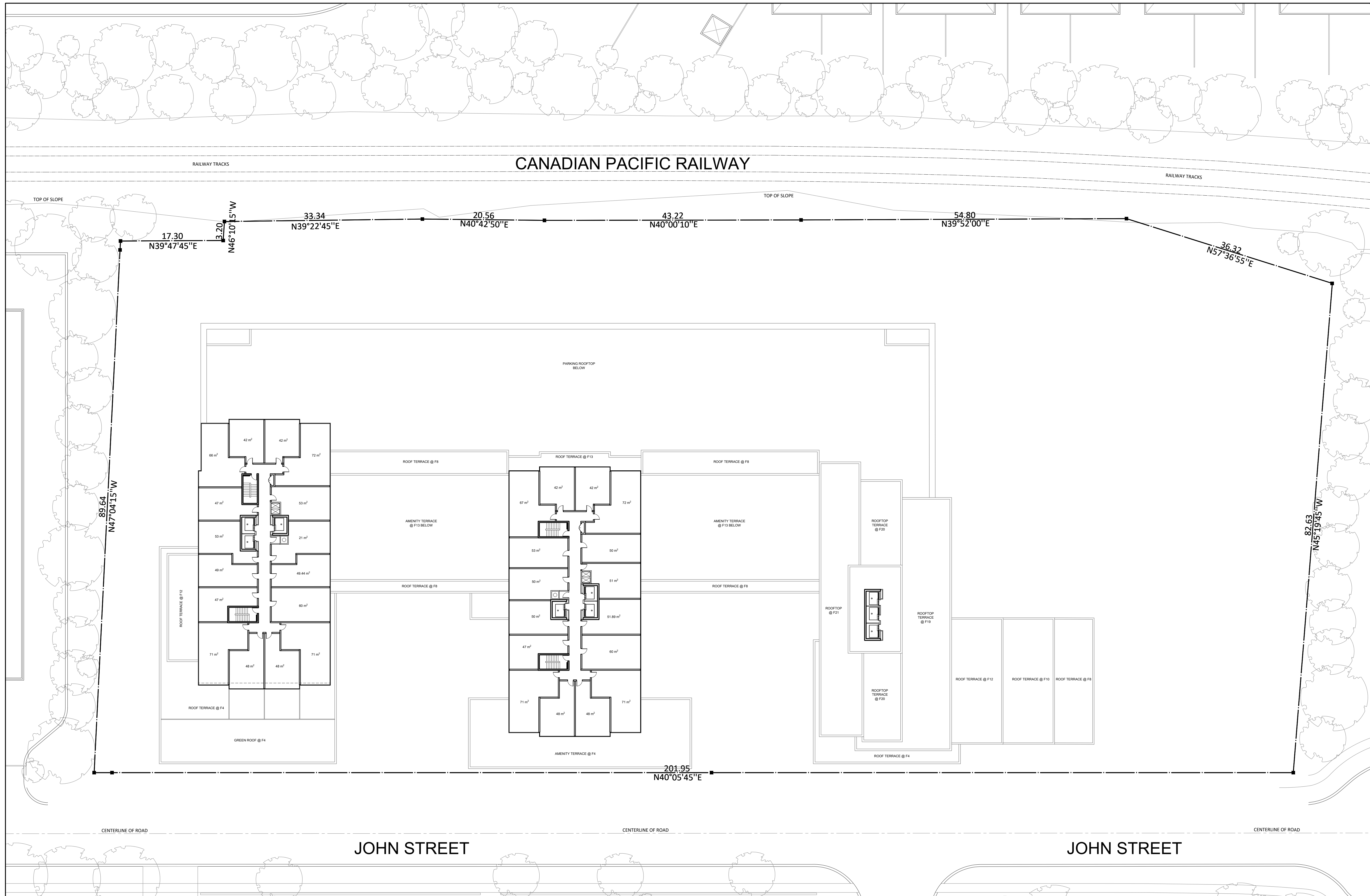
1 F21 FLOOR PLAN 1:300
