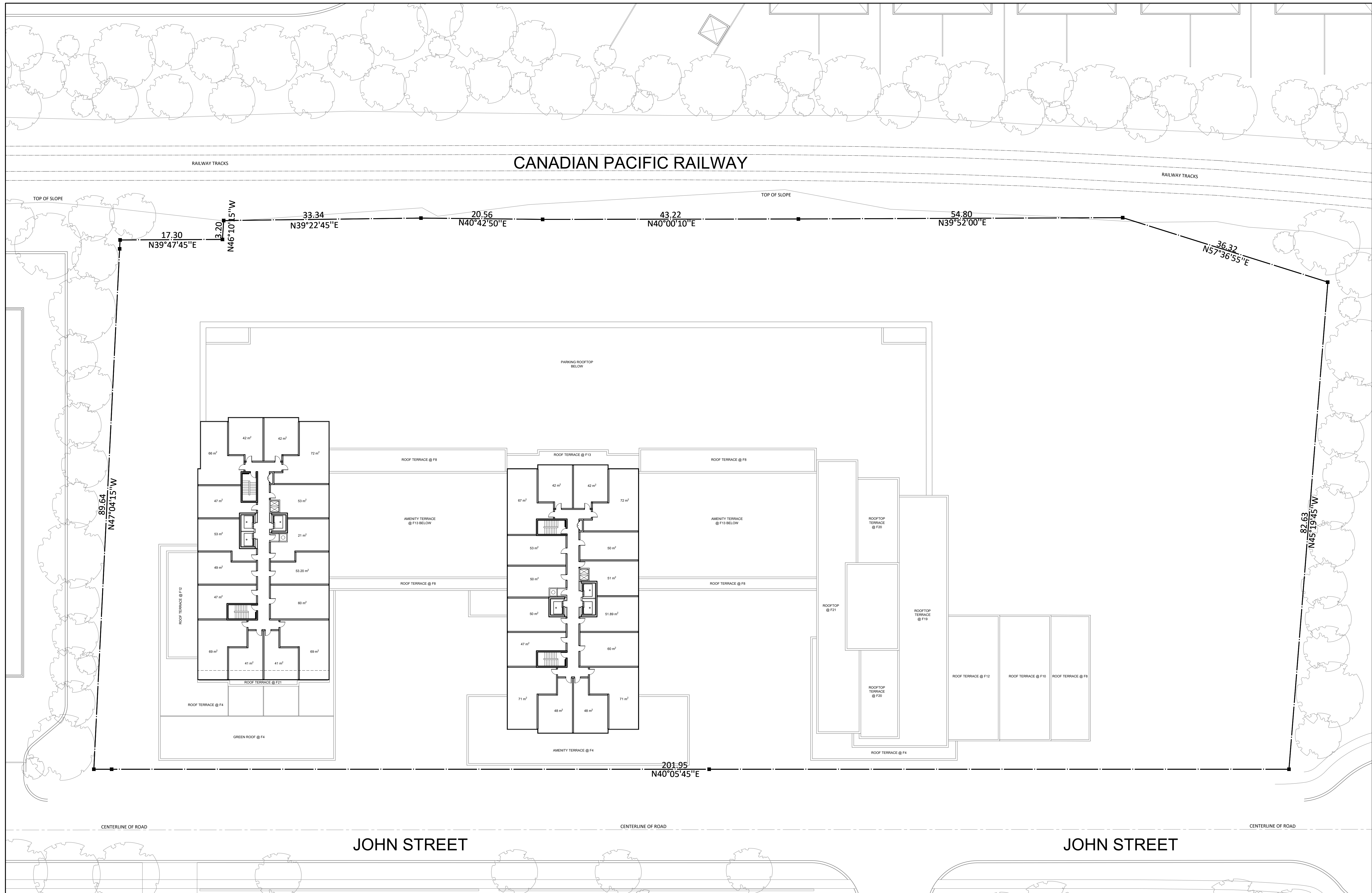
1 F22 FLOOR PLAN 1:300
