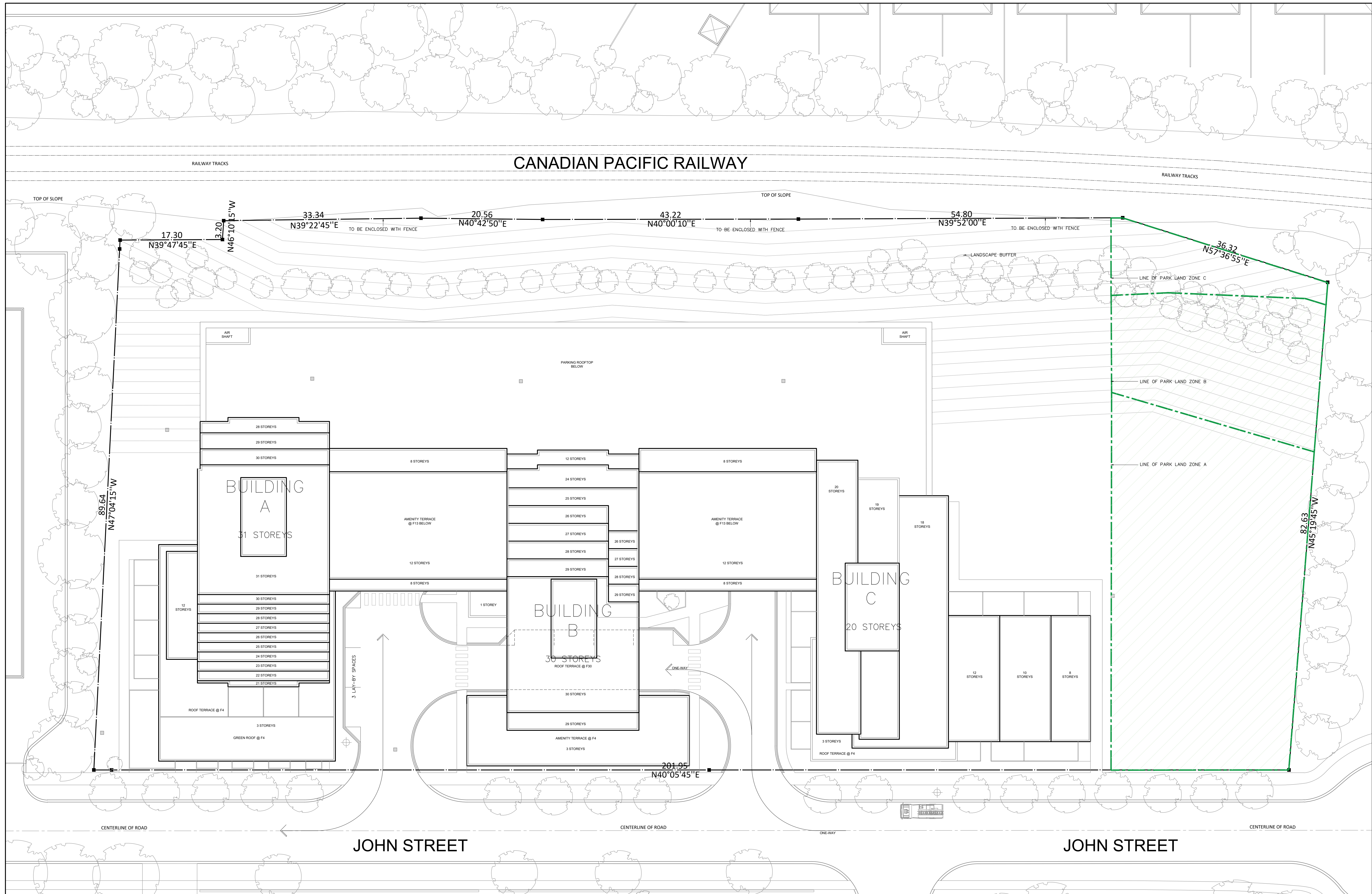
1 ROOF PLAN 1:300
