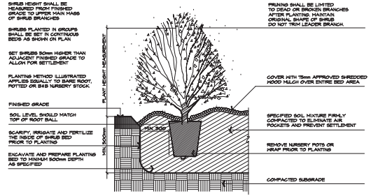
2 SHRUB PLANTING DETAIL TYPICAL INSTALLATION ABAL-P01-0217
