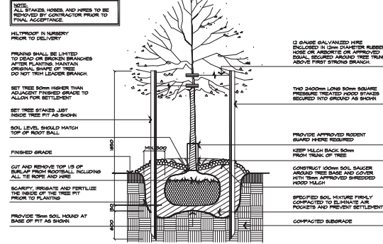
1 DECIDUOUS TREE PLANTING DETAIL TYPICAL INSTALLATION FOR 75mm CALIPER TREES OR LESS ABAL-P01-0214
