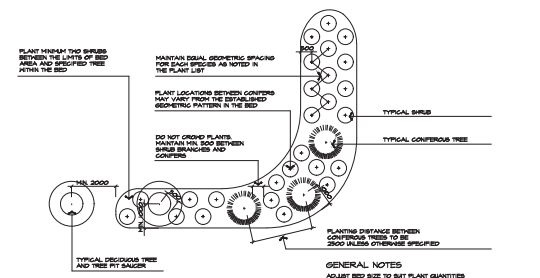
3 TYPICAL PLANTING LAYOUT - LAWN AREA SYMBOLS REPRESENT INSTALLED PLANT SIZE ABAL-P01-0218
