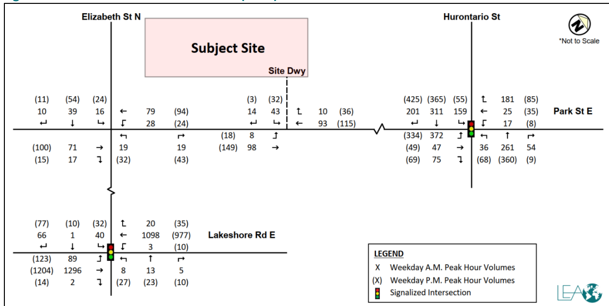
Figure 4-2: Future Total Traffic Volumes (2030)
