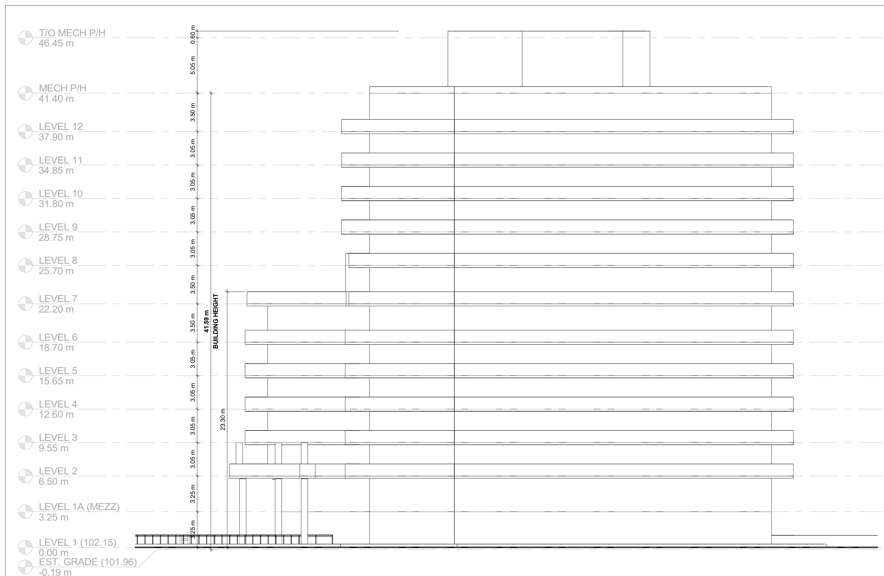
2 WEST ELEVATION 1 : 200
