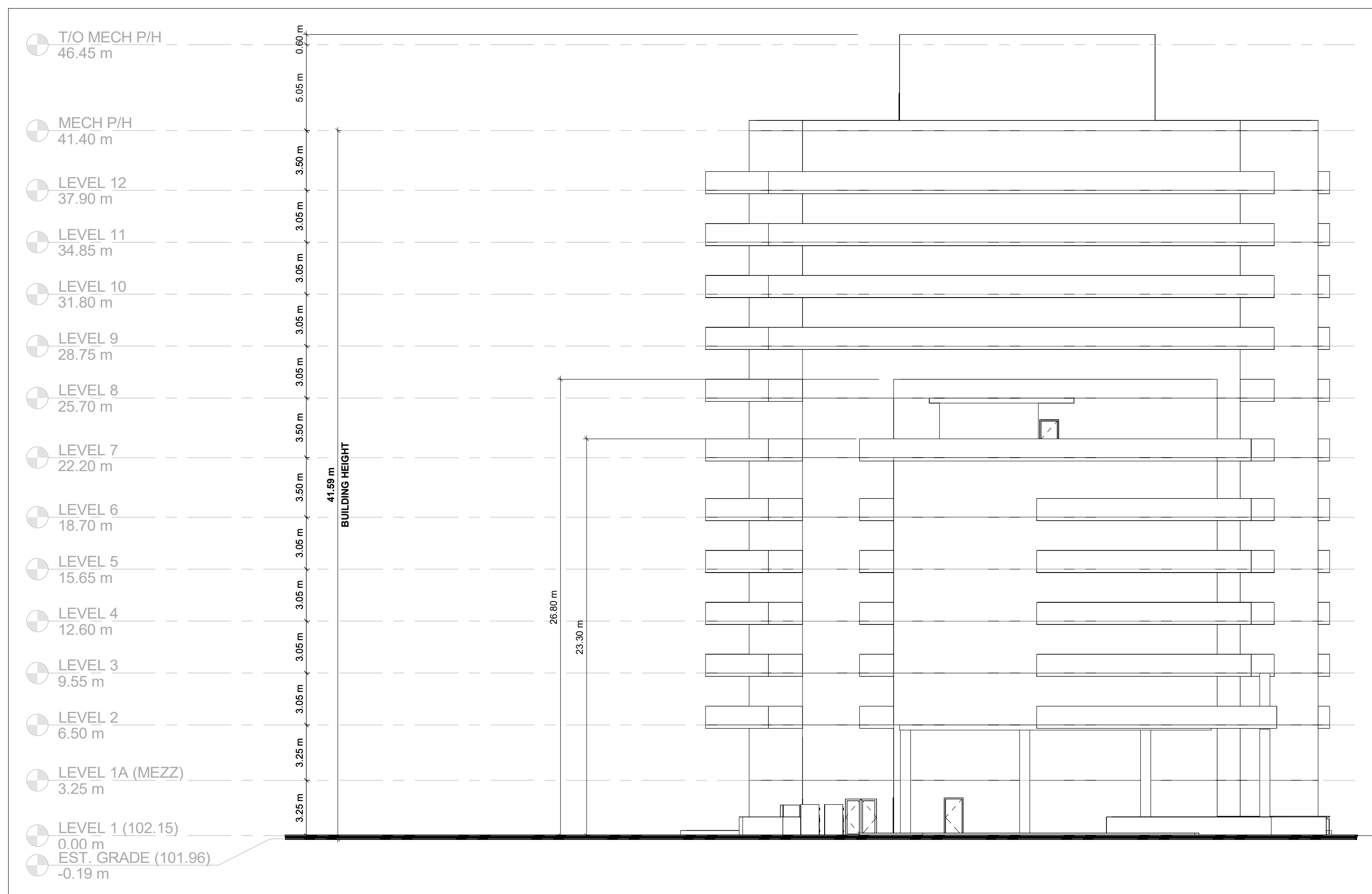
1 EAST ELEVATION 1 : 200
