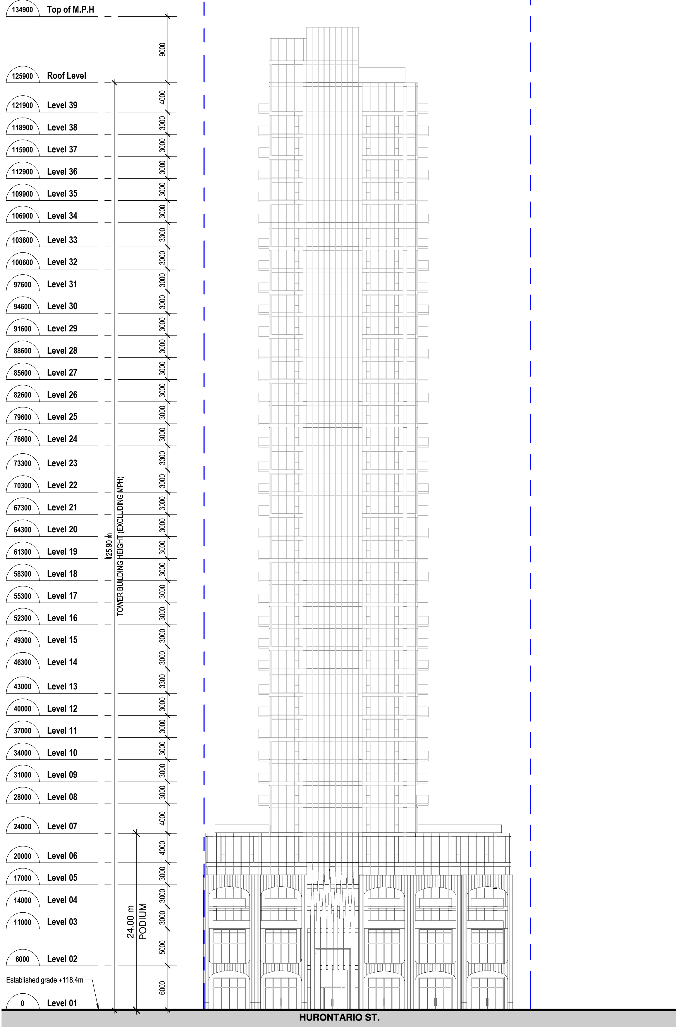
1 ZBA_Building Elev_South AZ401 1:300
