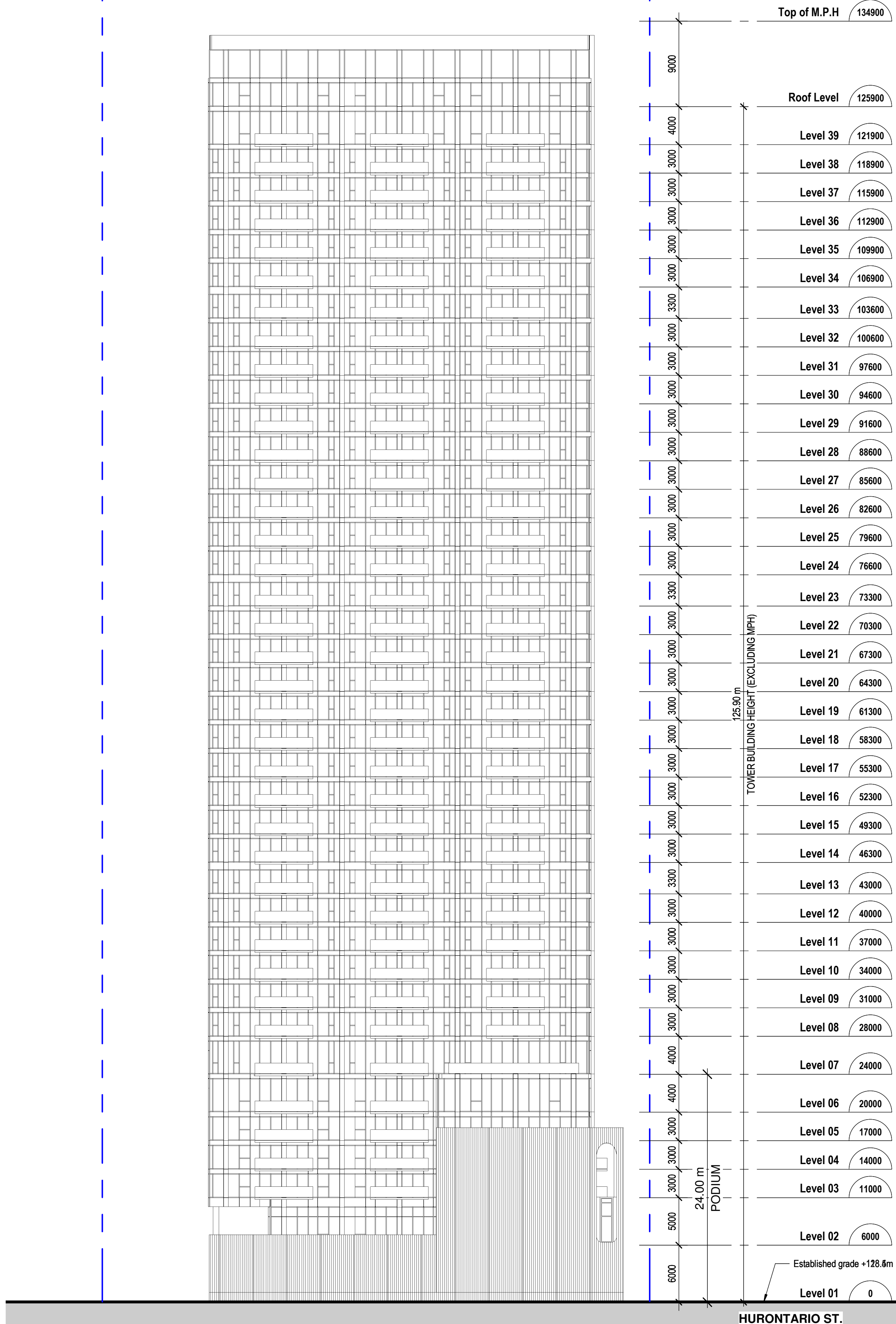
2 ZBA_Building Elev_West AZ401 1:300
