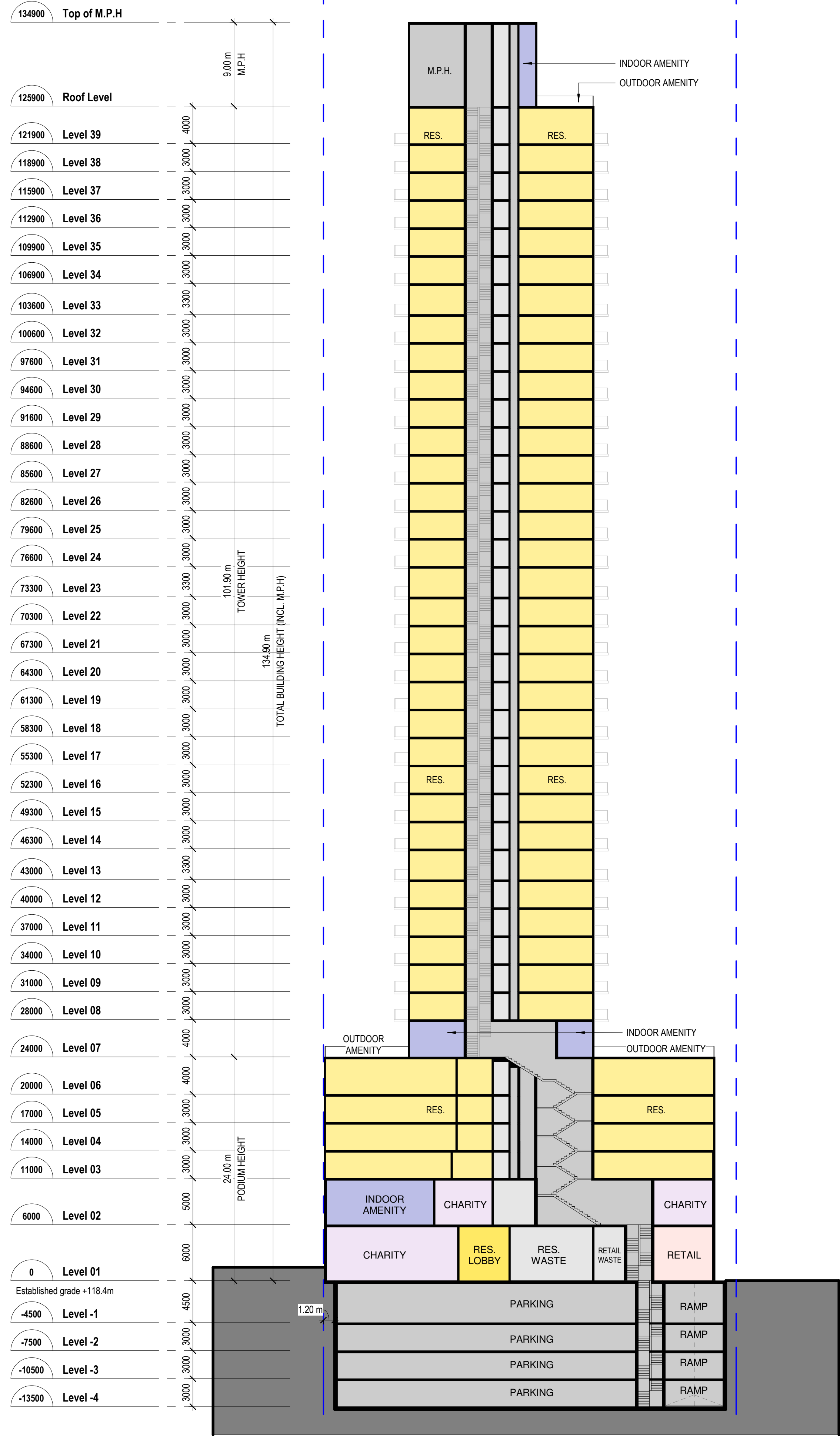
1 ZBA_Building Section_North AZ501 1 : 300
