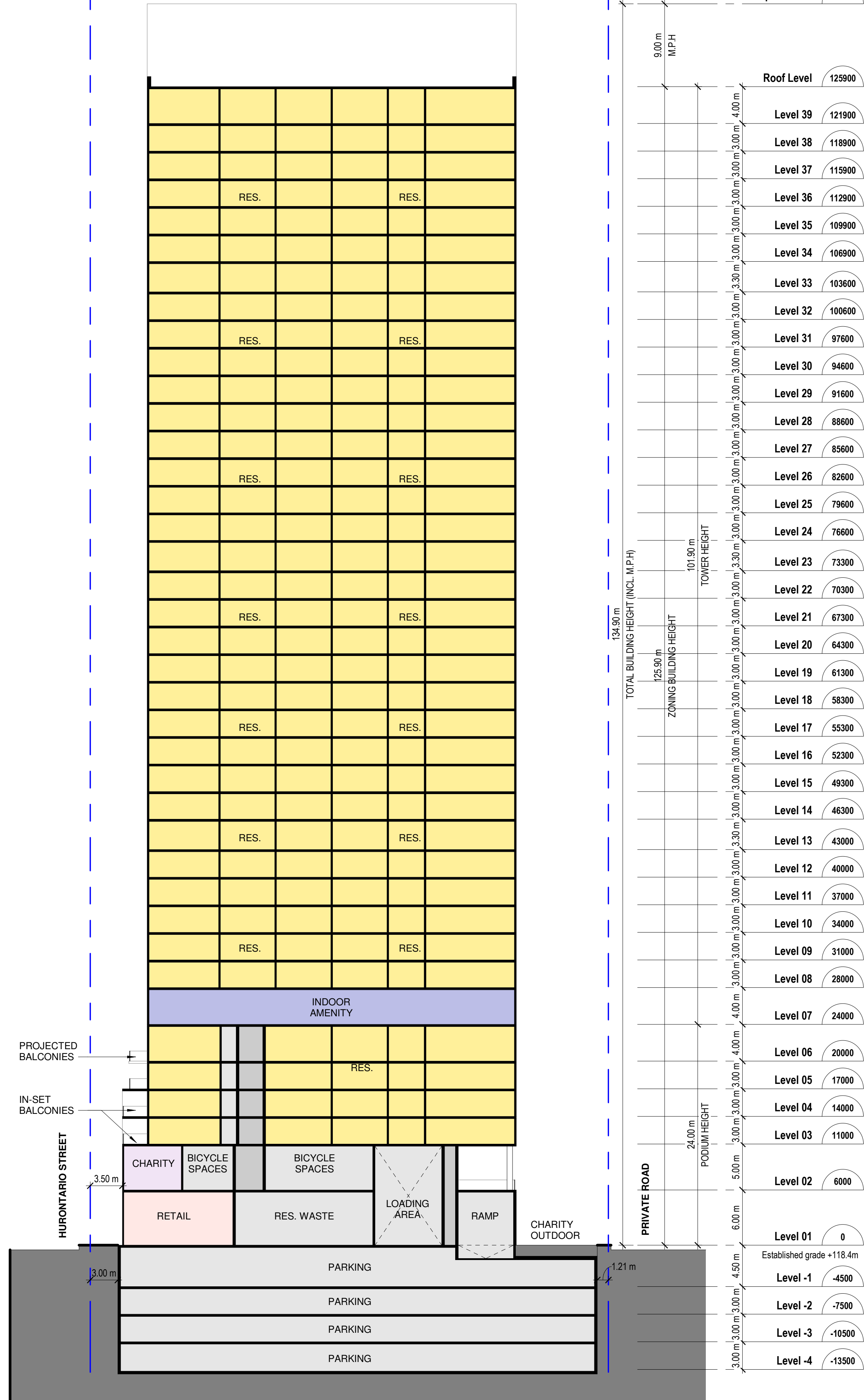
2 ZBA_Building Section_East AZ501 1 : 300
