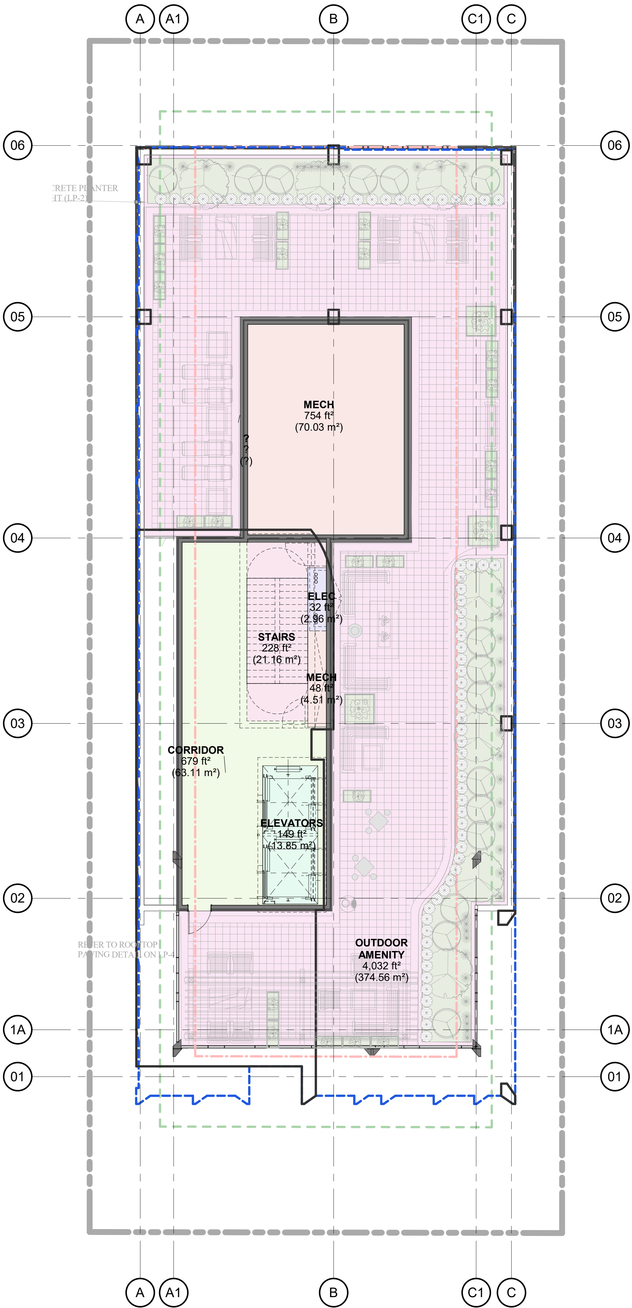
1 T/O ROOF DECK A103 1 : 100
