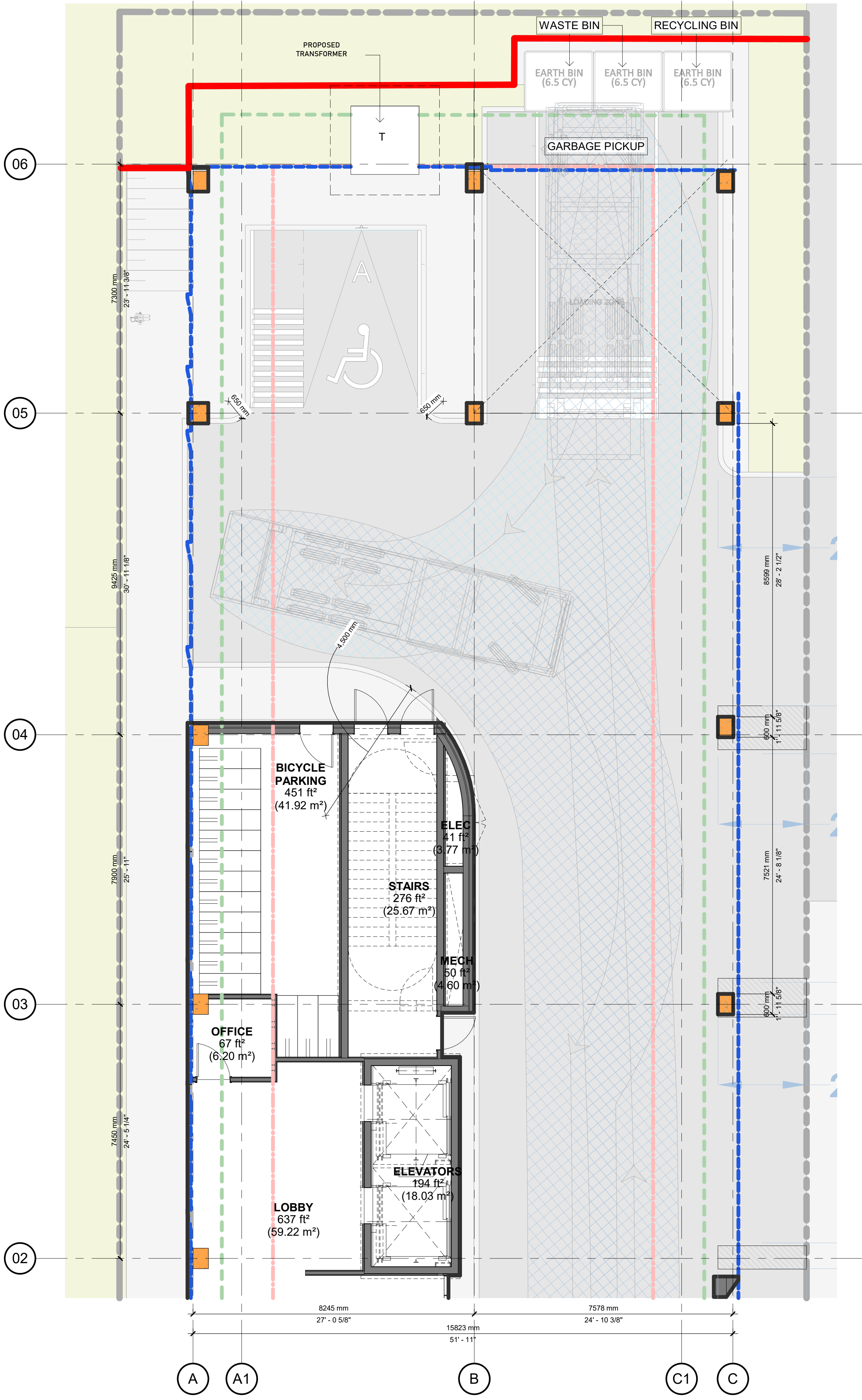
1 WASTE MANAGEMENT PLAN A104 1 : 75
