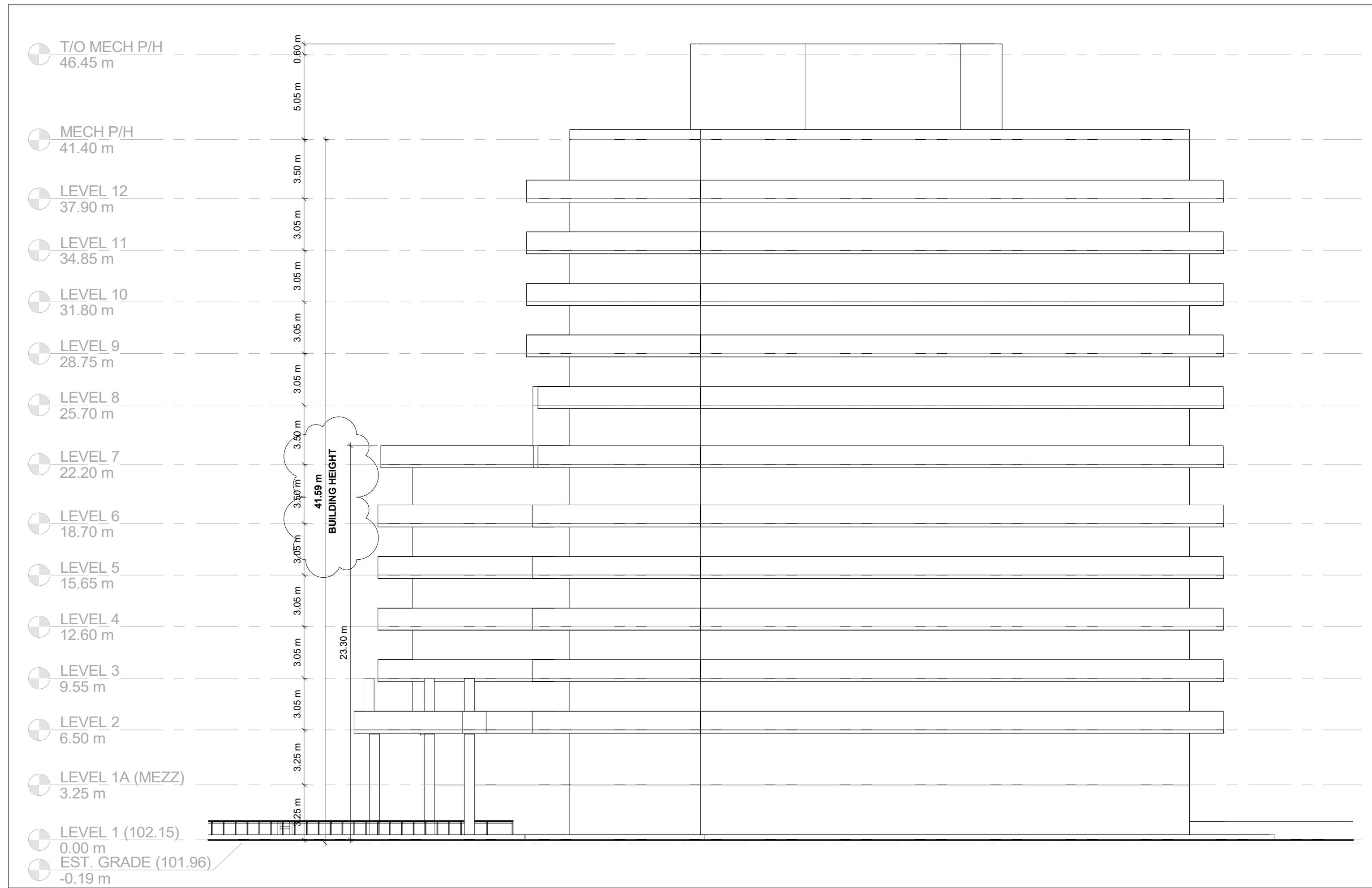
2 WEST ELEVATION 1 : 200
