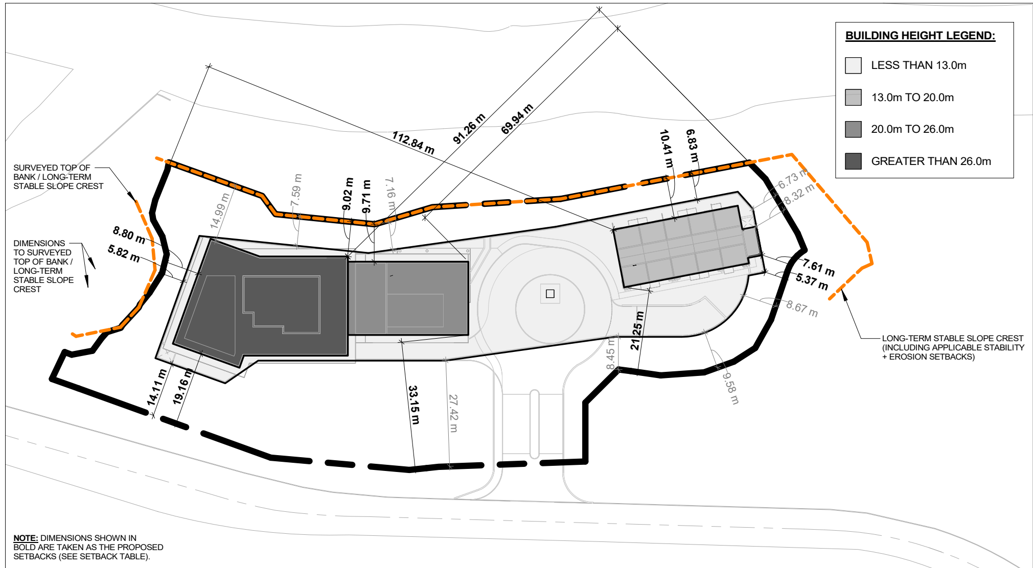
② HEIGHT & SETBACK DIAGRAM 1 : 1000
