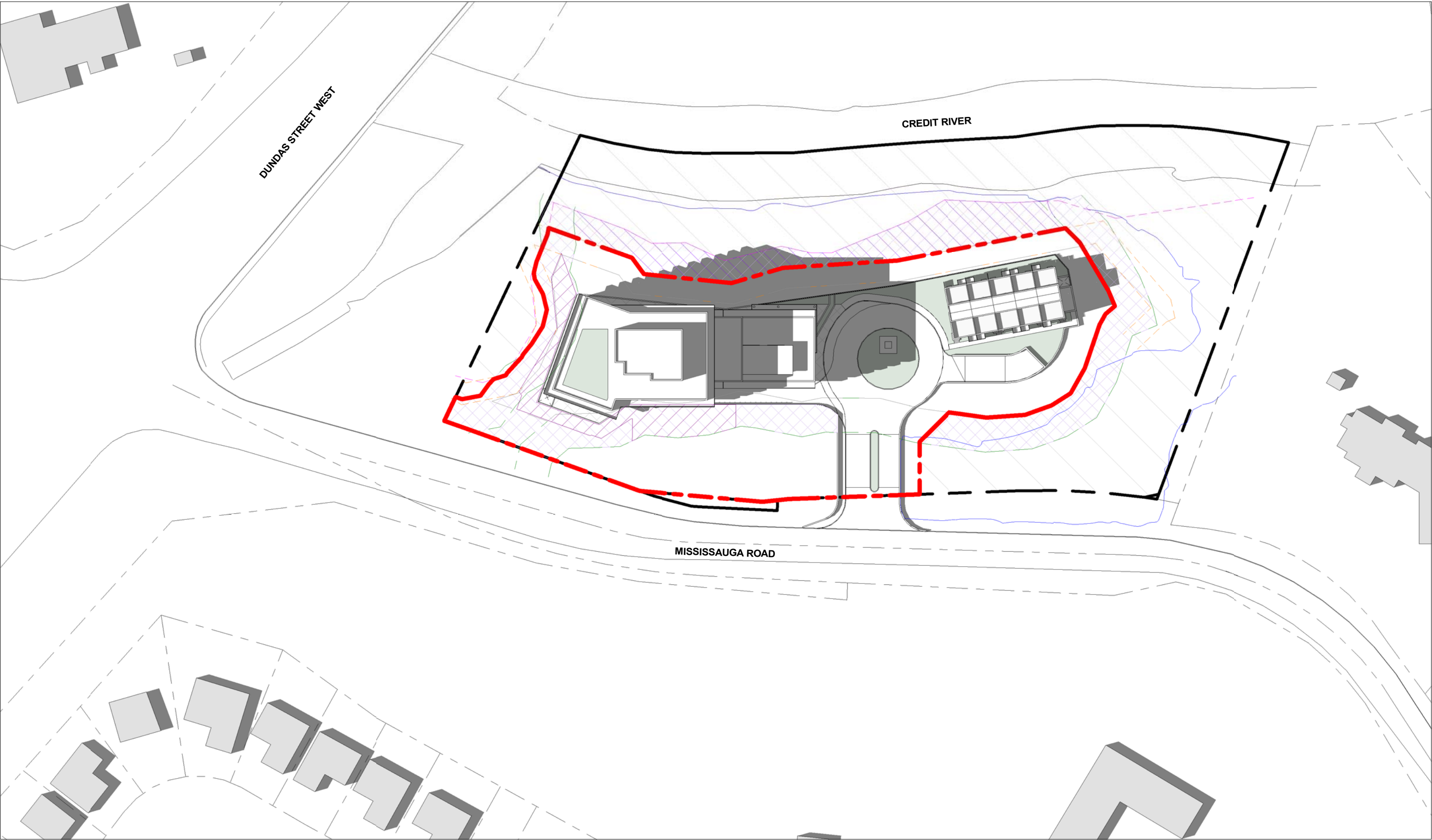
4 JUNE 21 - 17.20 PM 1 : 1000
