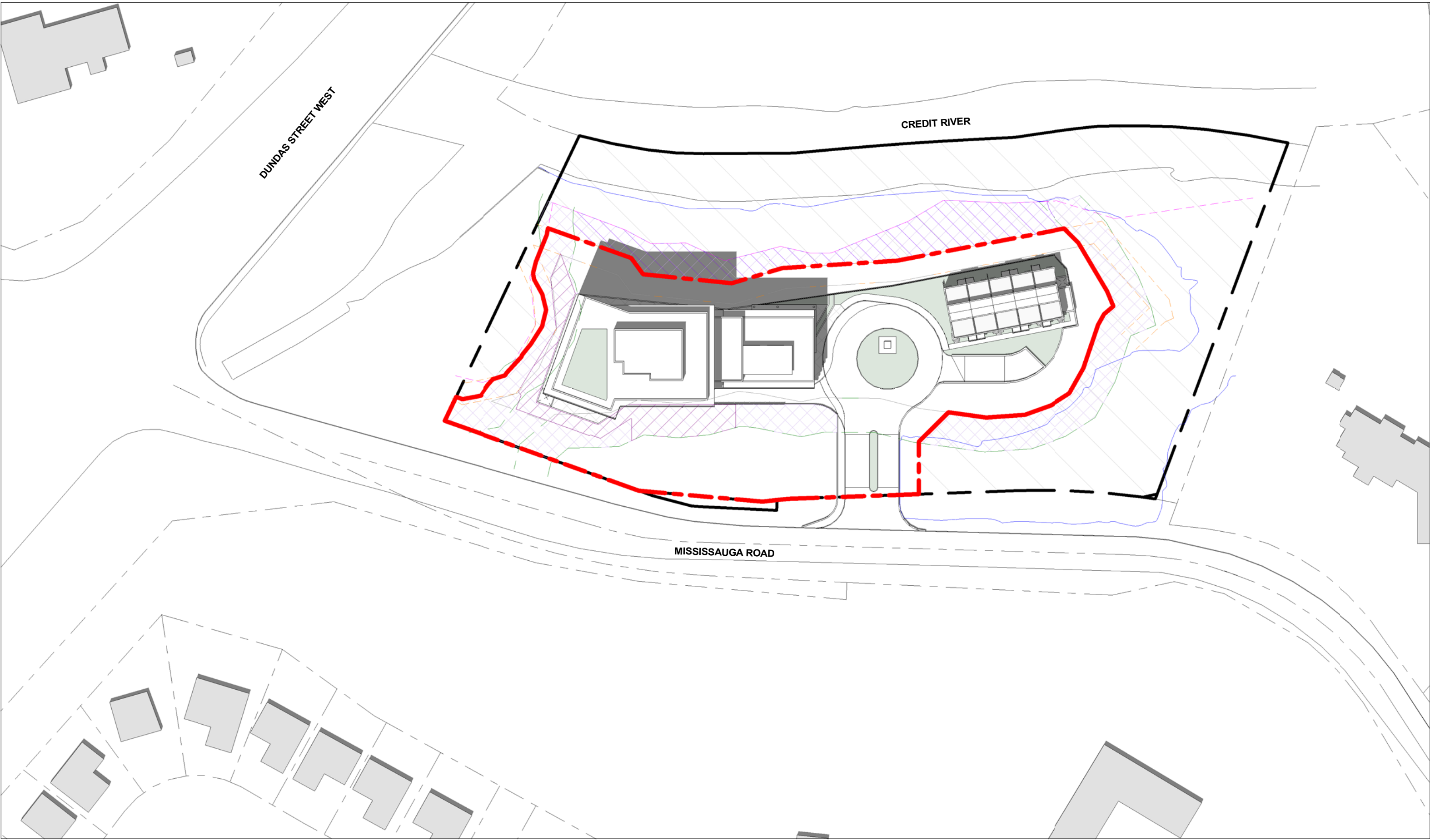
1 JUNE 21 - 14.20 PM 1 : 1000
