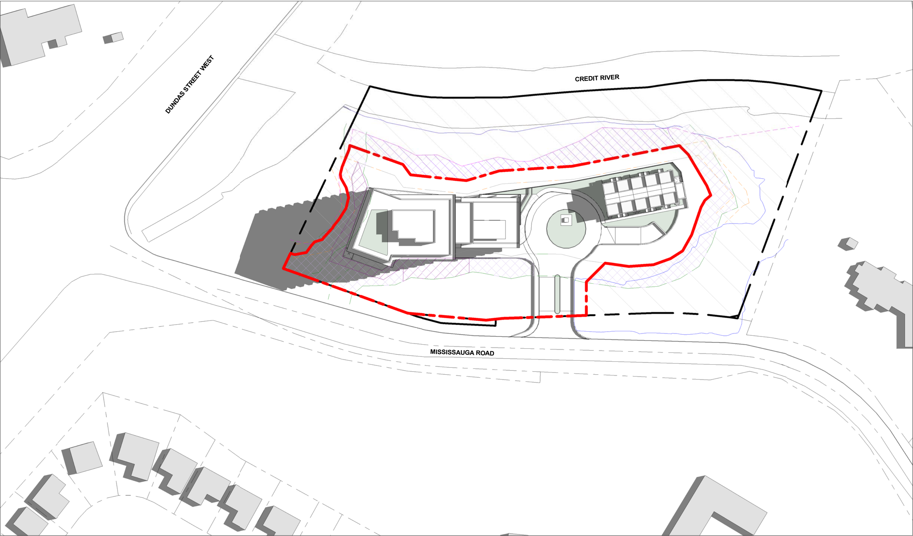
4 JUNE 21 - 9.20 AM 1 : 1000
