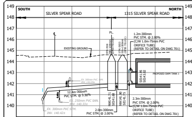
SECTION 1-1 (STORM SERVICE CONNECTION) H = 1:200 V = 1:100
