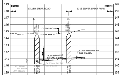
SECTION 2-2 (SANITARY SERVICE CONNECTION) H = 1:200 V = 1:100
