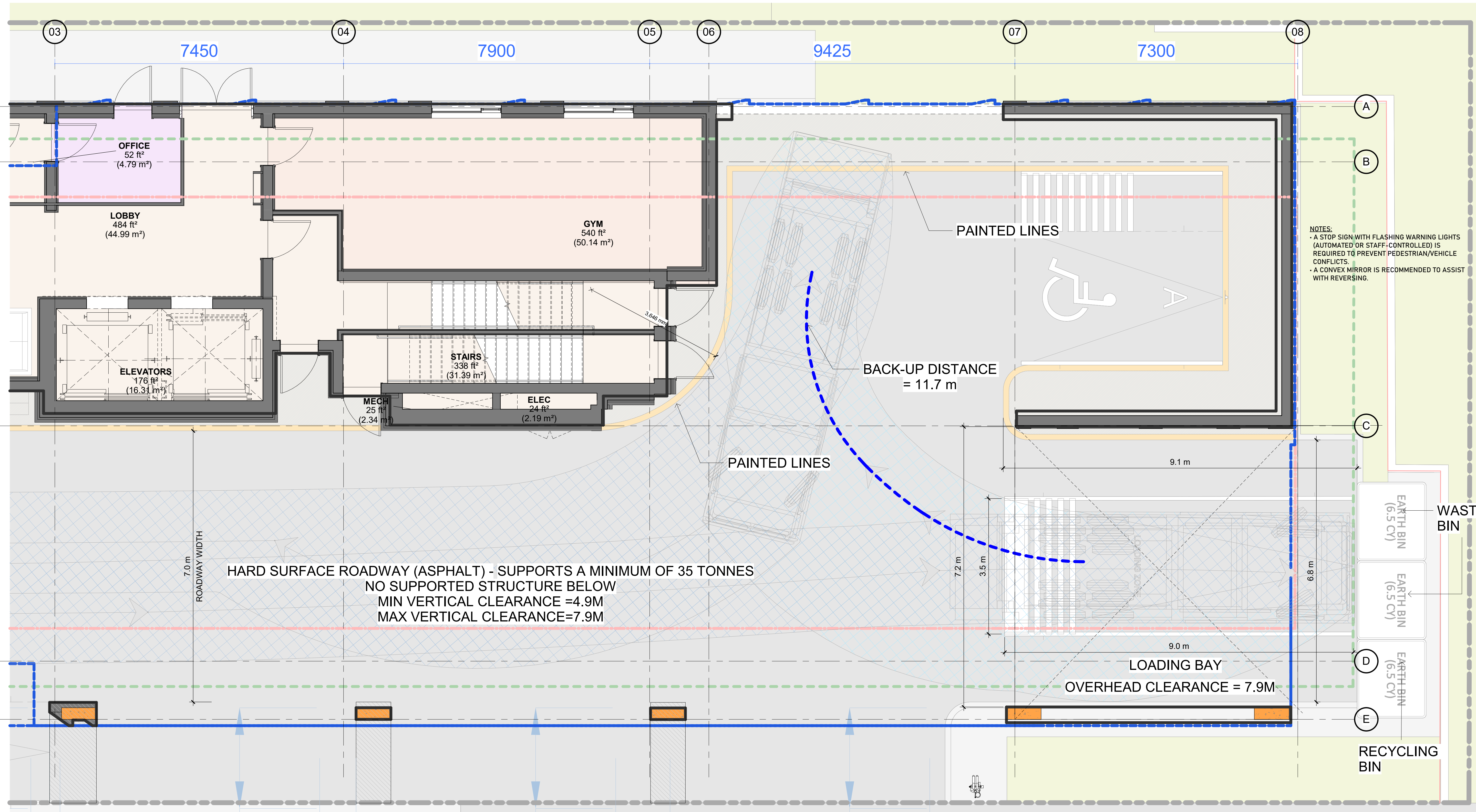
1 WASTE MANAGEMENT PLAN A104 1: 50
