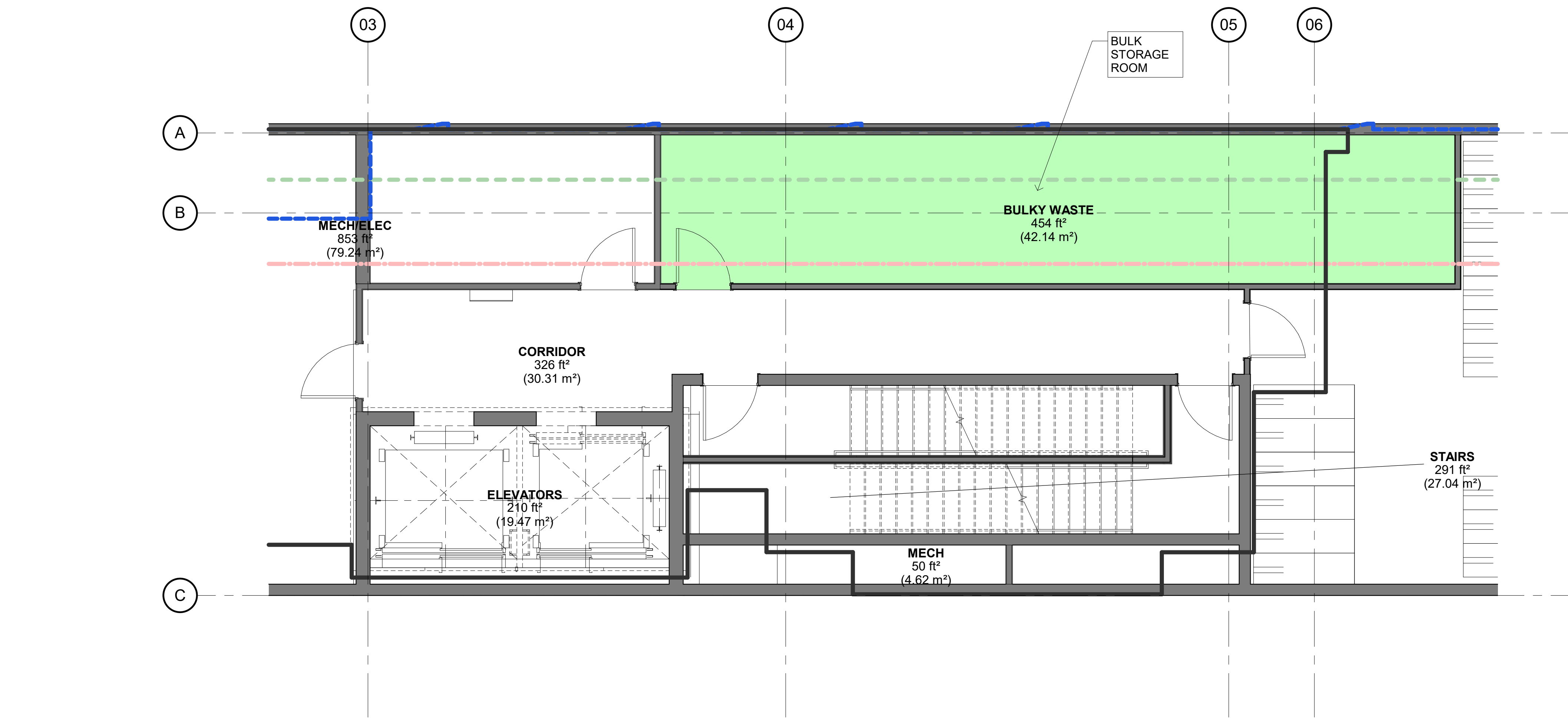
2 BASEMENT - WASTE MANAGEMENT PLAN A104 1: 50
