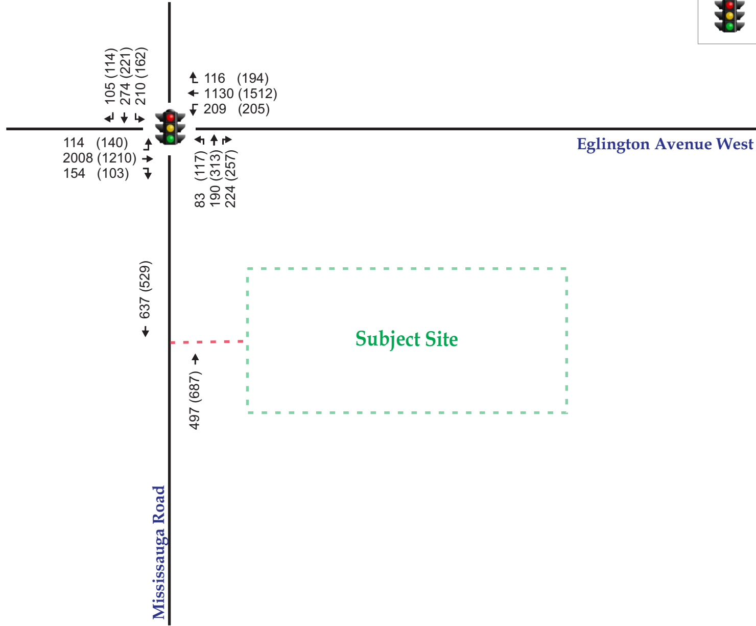
Figure 10 - Future (2029) Background Traffic Volumes
