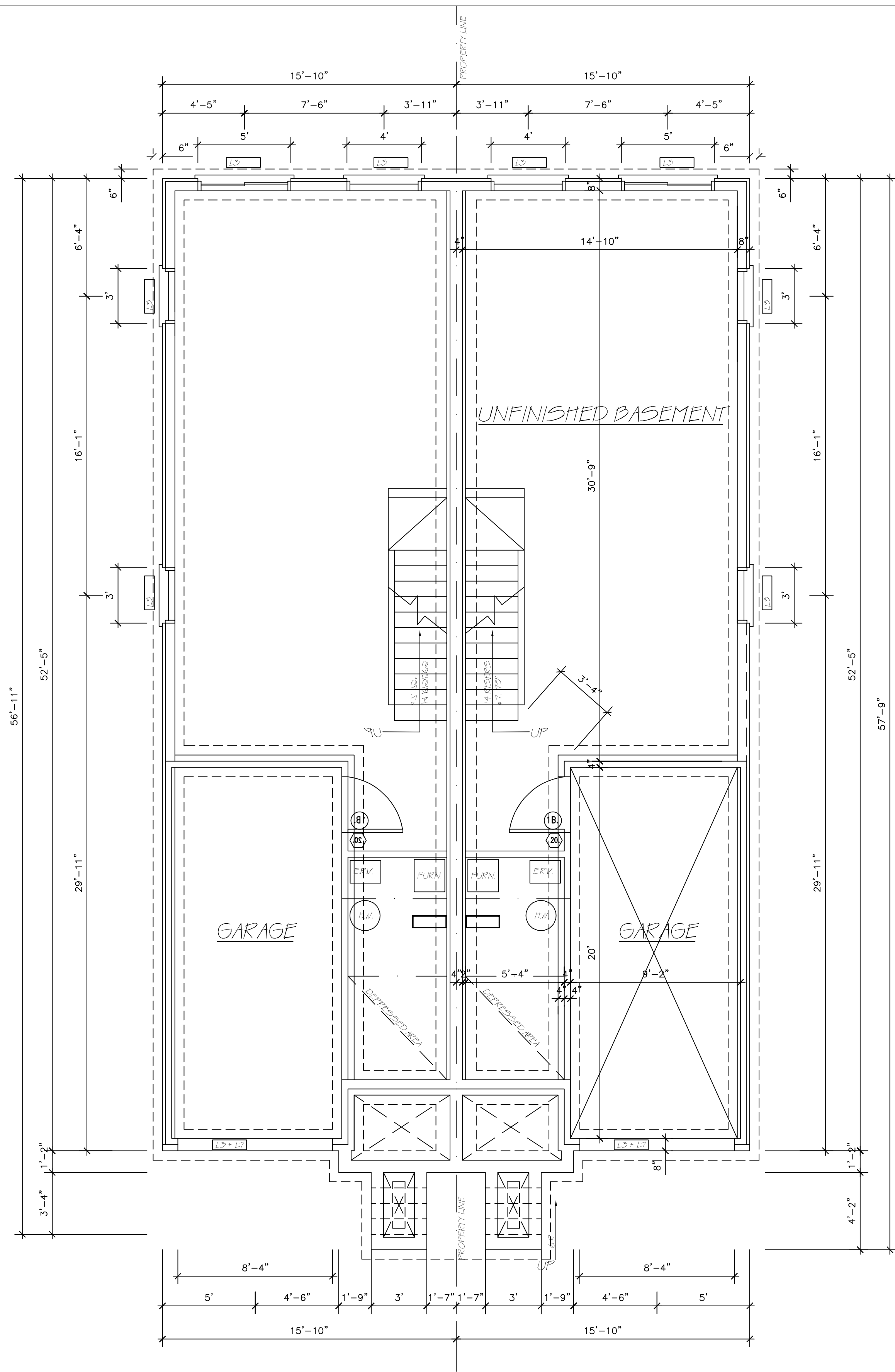
BASEMENT PLAN
