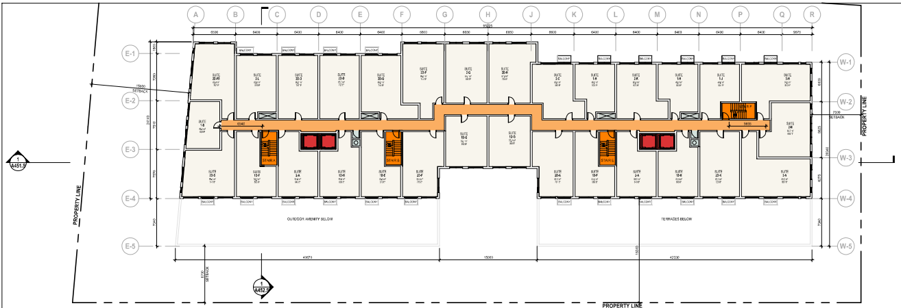
3RD & 6TH FLOOR PLAN
