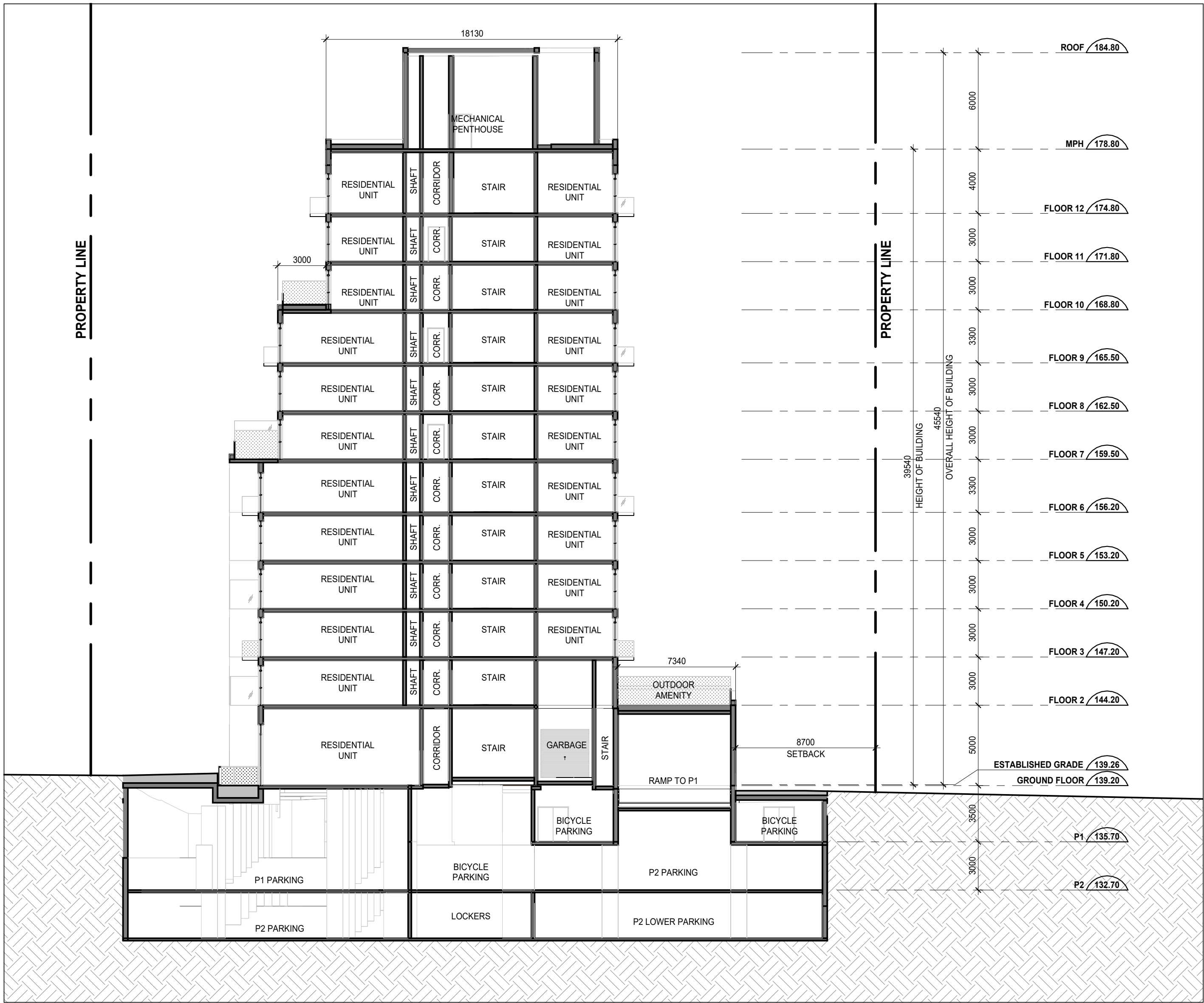
1 NORTH-SOUTH SECTION A452.S
