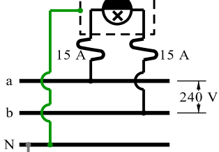
SCHEMATIC 2 240 V (NOTE 4)
