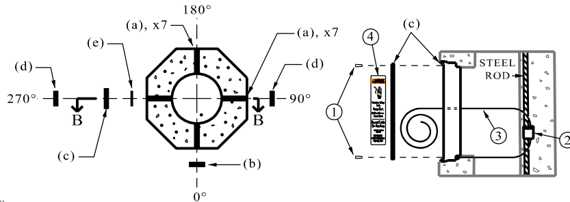
SECTION A-A (STEEL RODS NOT SHOWN)
