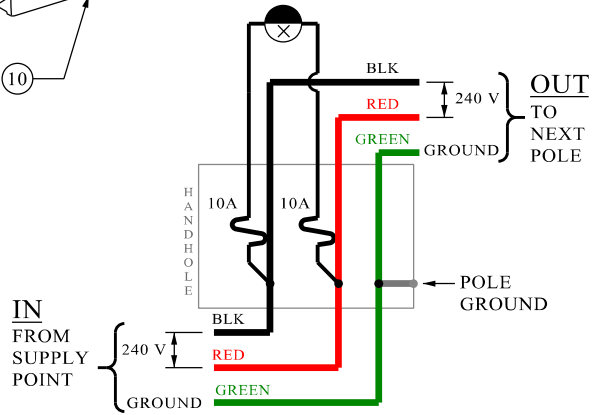
SCHMATIC DIAGRAM
