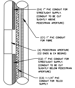
DETAIL 1 PEDESTRIAN APERTURE
