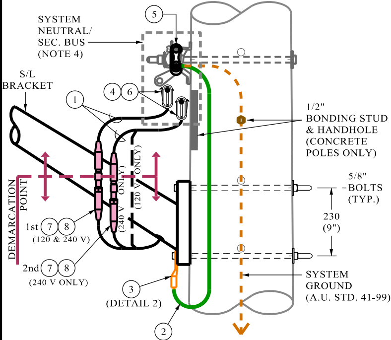
DETAIL 1 S/L CONNECTION
