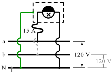
SCHEMATIC 1 120 V (NOTE 4)
