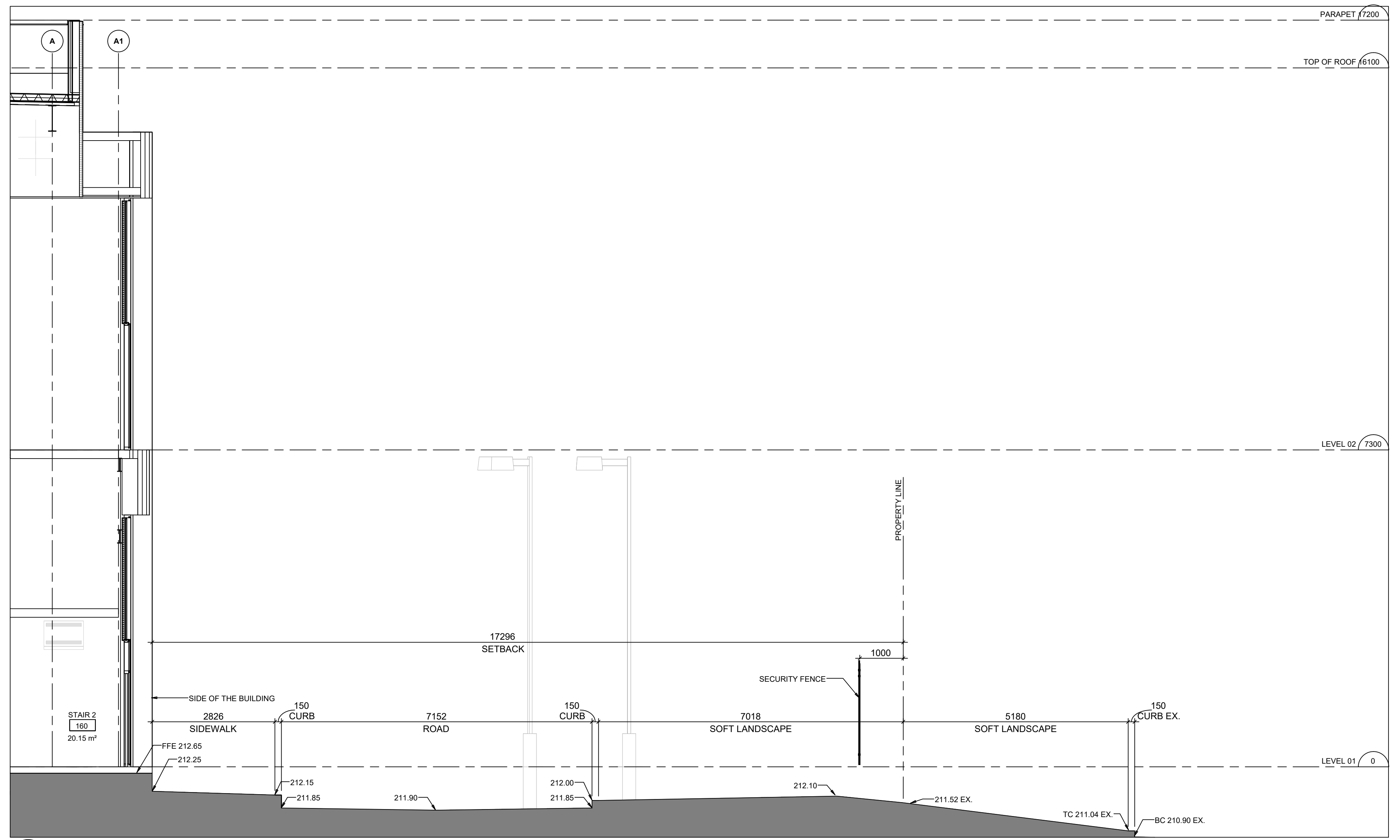
1 BOULEVARD CROSS SECTIONS SOUTH SIDE A410 1:50
