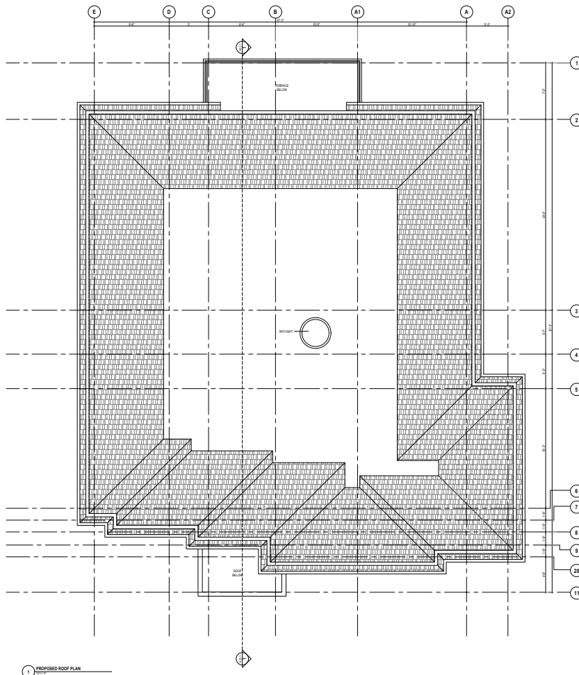
1 PROPOSED ROOF PLAN
