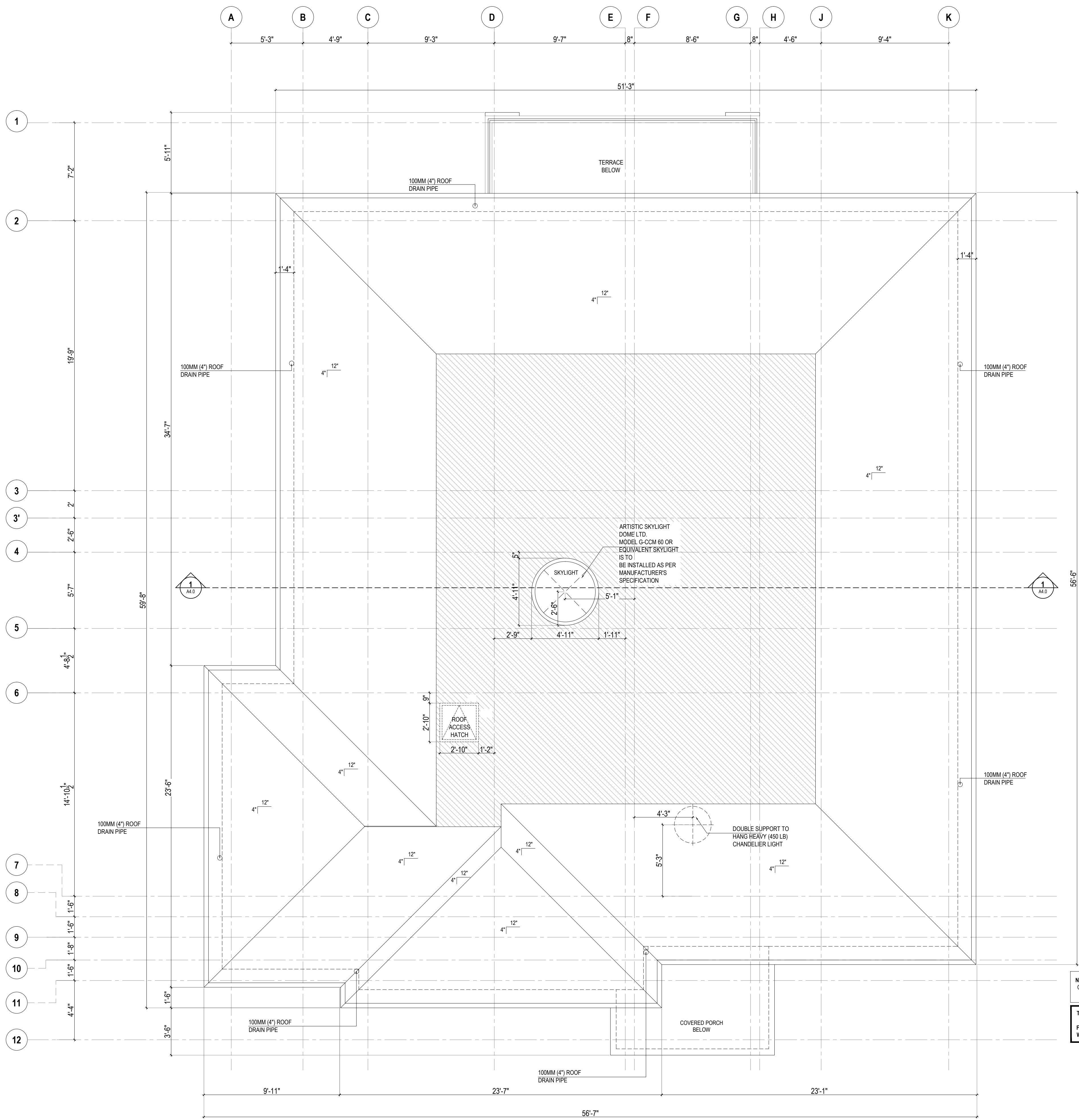
5 ROOF PLAN 1/4"=1'-0"
