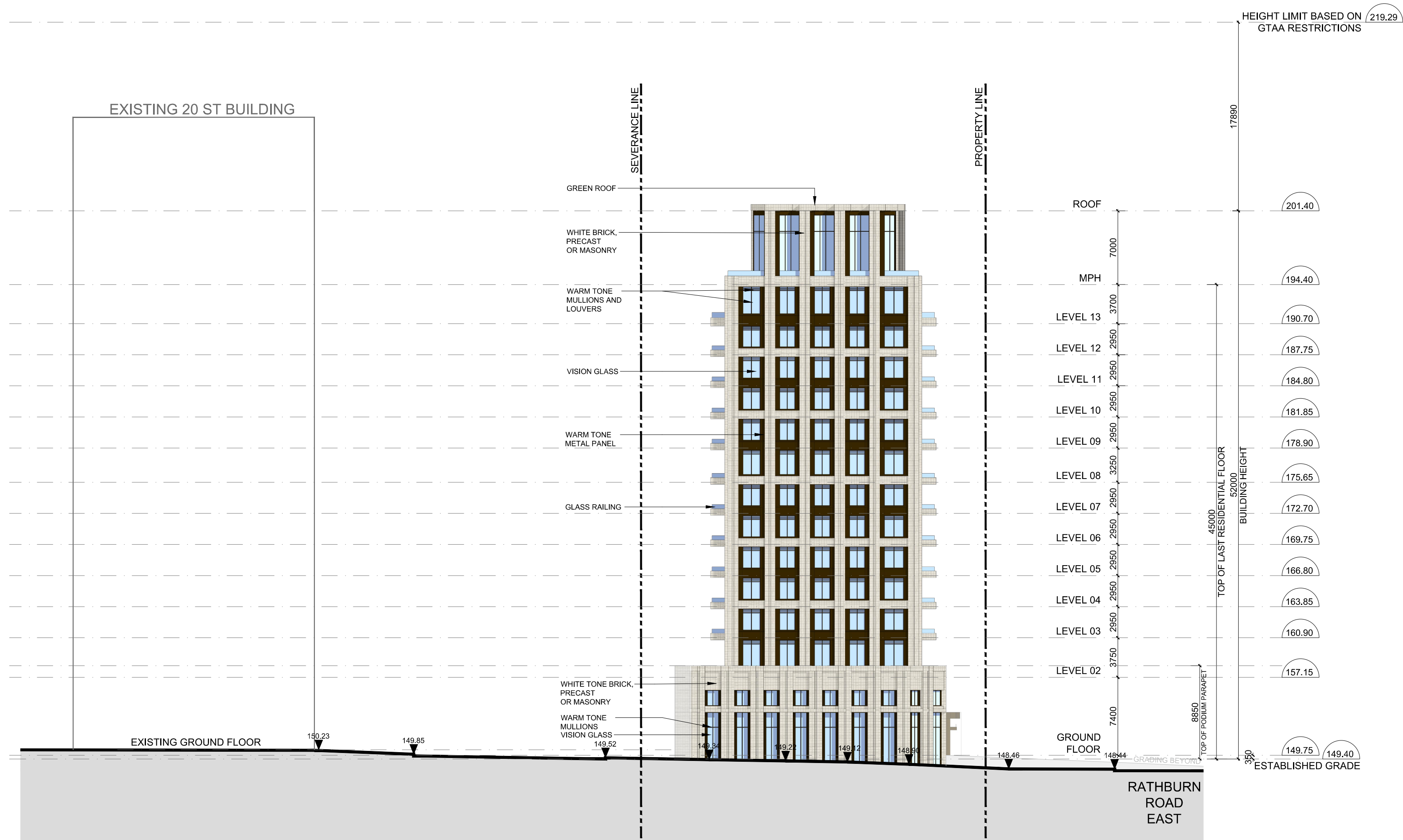
SOUTH ELEVATION
