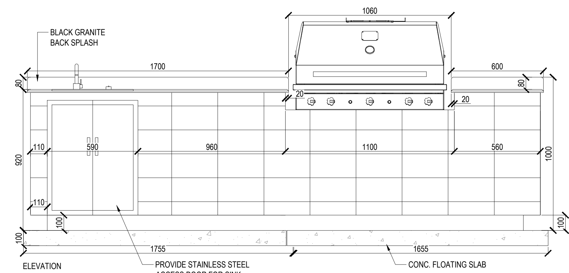
5 OUTDOOR KITCHEN OR APPROVED EQUAL SCALE 1:15
