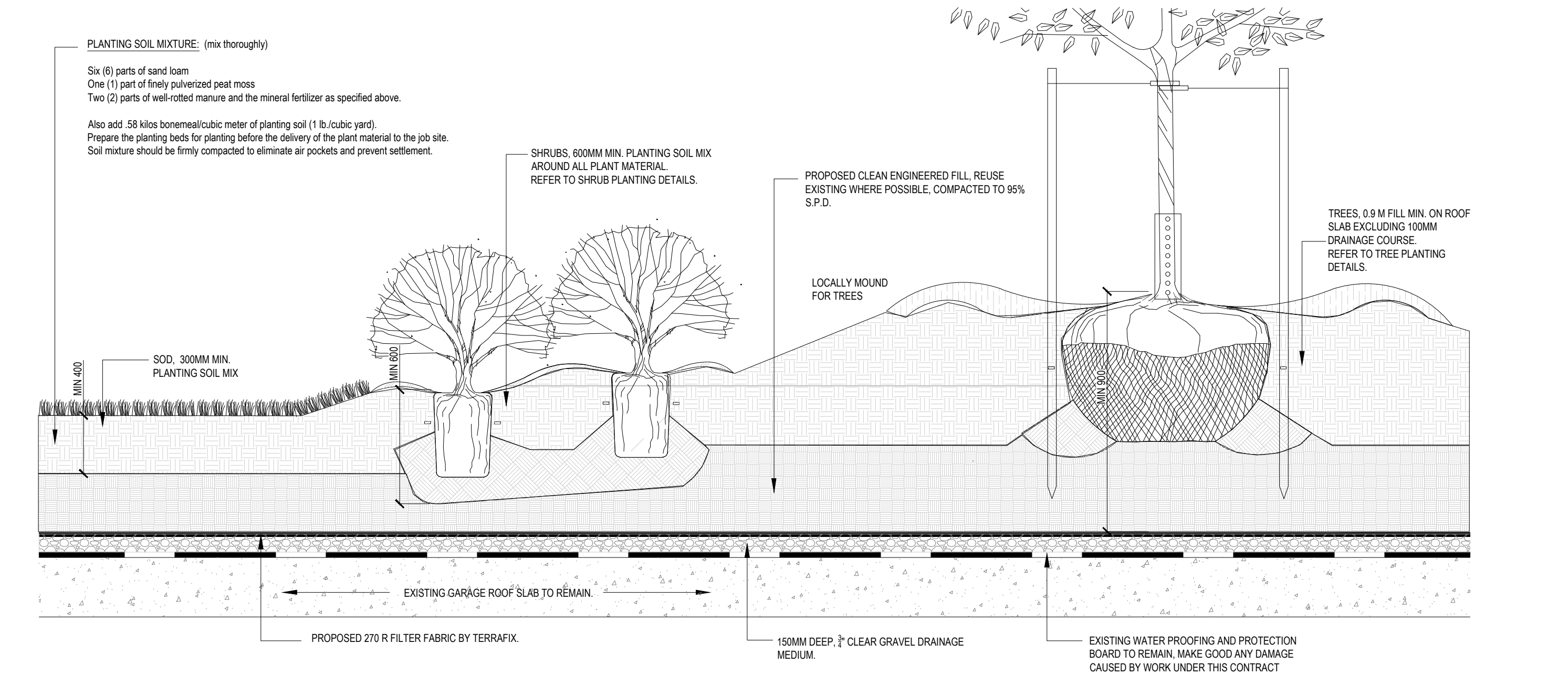
5 PLANTING ON SLAB DETAIL SCALE = N.T.S.
