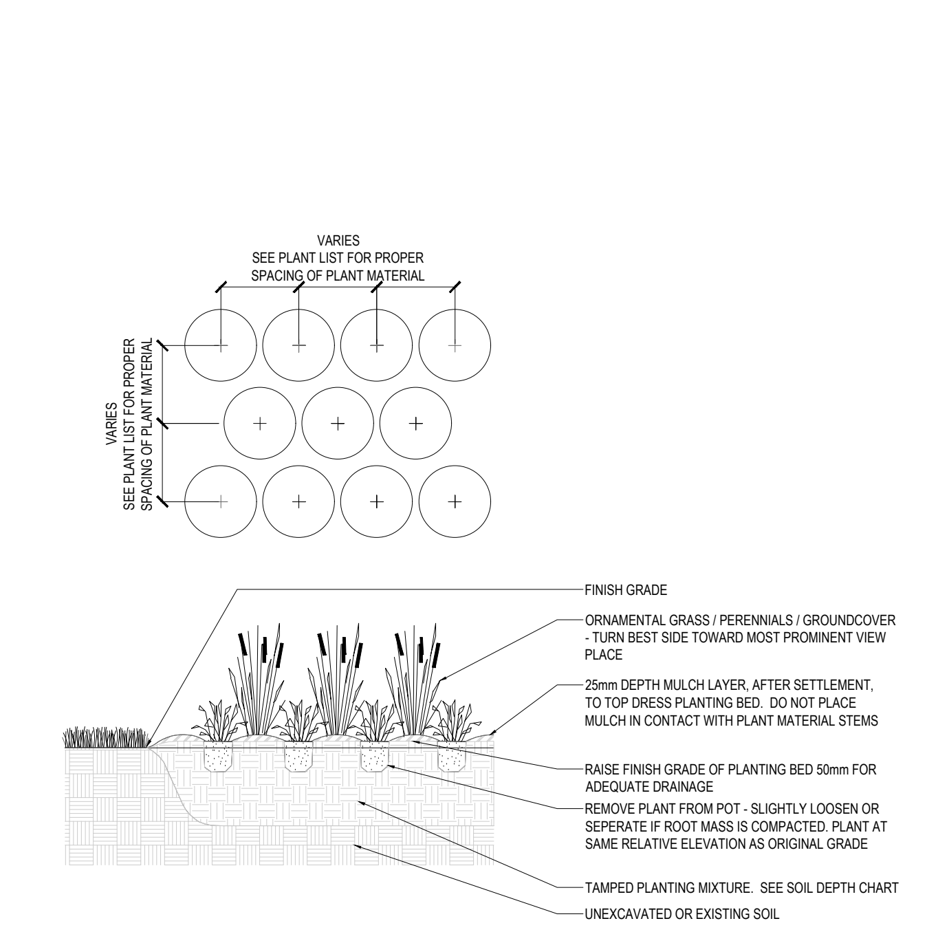
3 GROUNDCOVER PLANTING DETAIL NO SCALE
