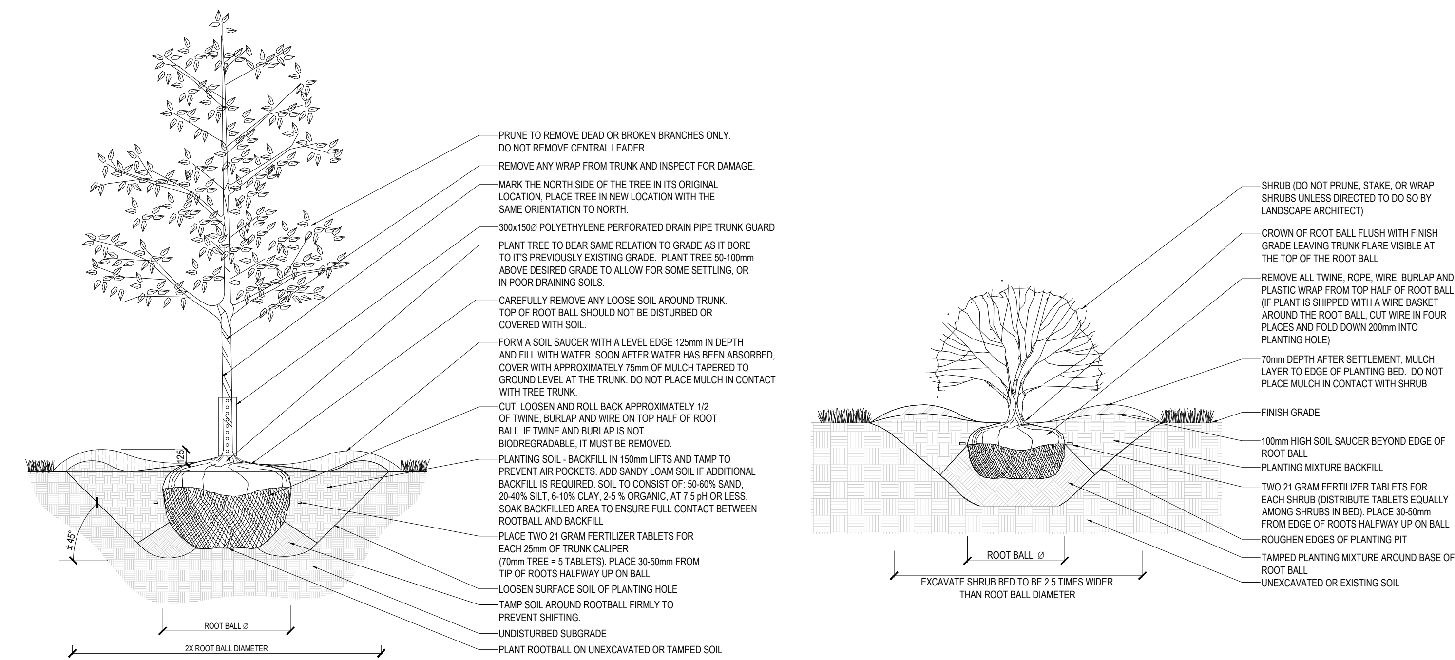
1 B&B DECIDUOUS TREE PLANTING DETAIL SCALE = N.T.S.
