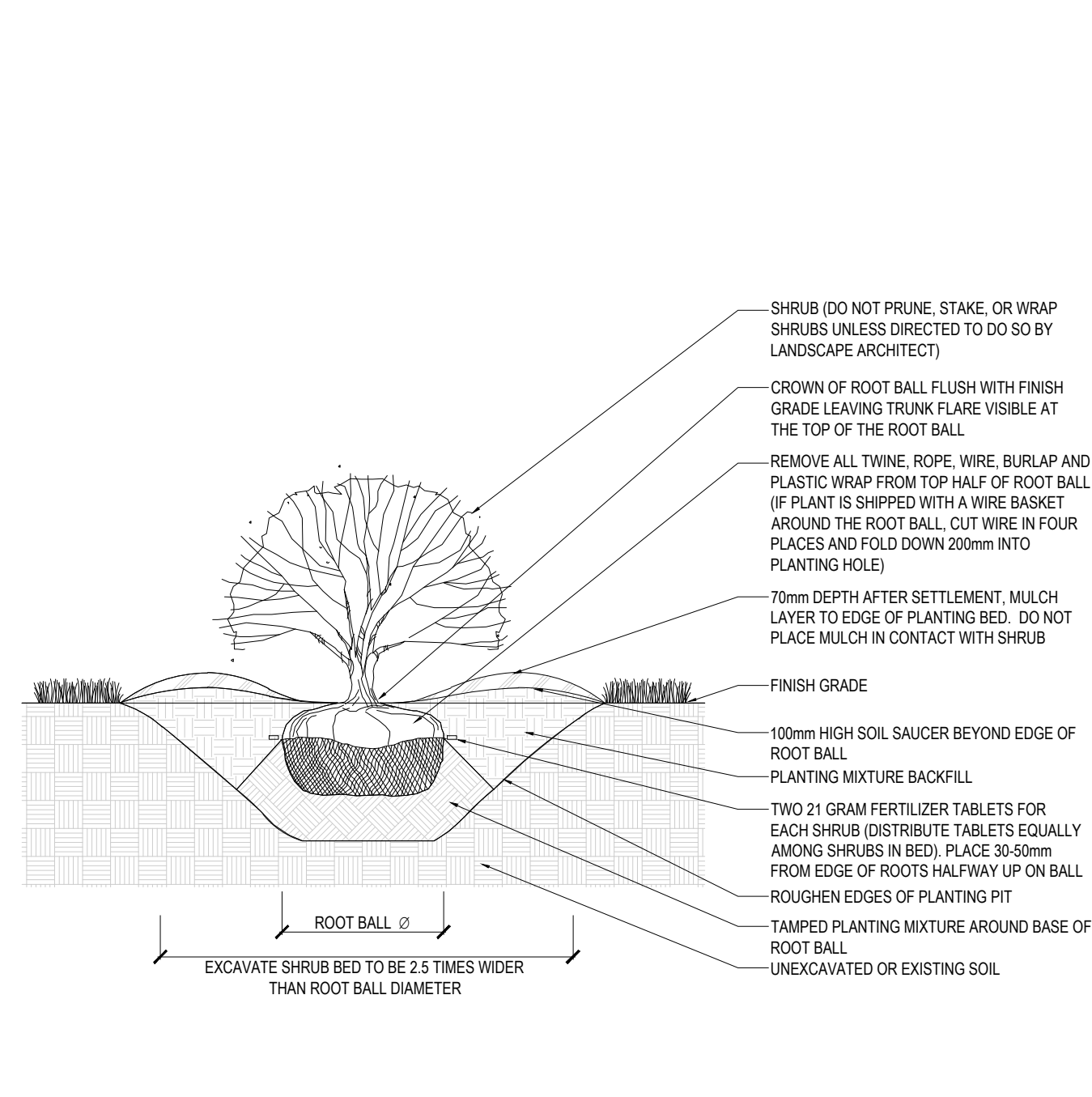
2 B&B SHRUB PLANTING DETAIL SCALE=NO SCALE
