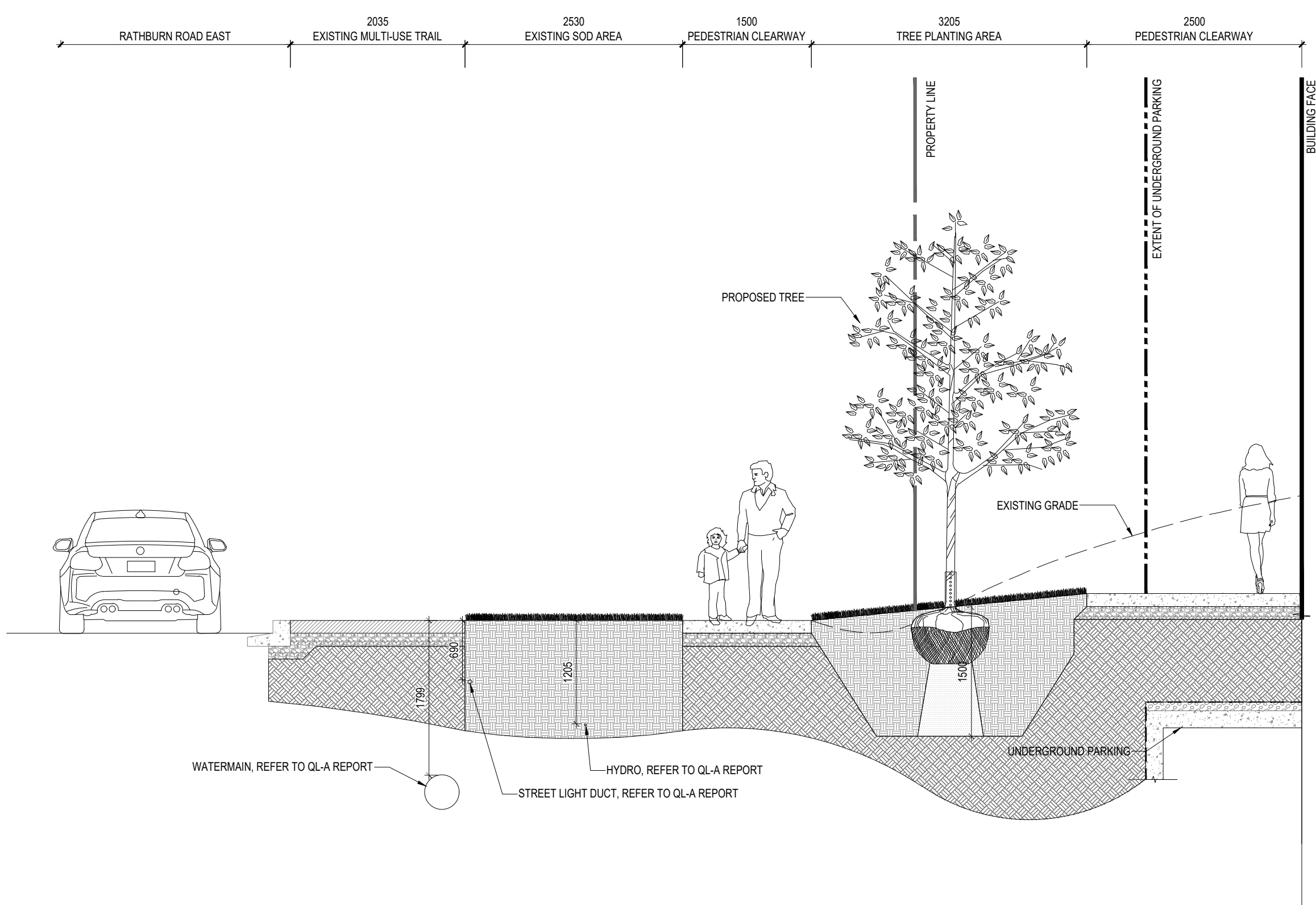
2 LANDSCAPE SECTION 2 RATHBURN ROAD EAST 1:50
