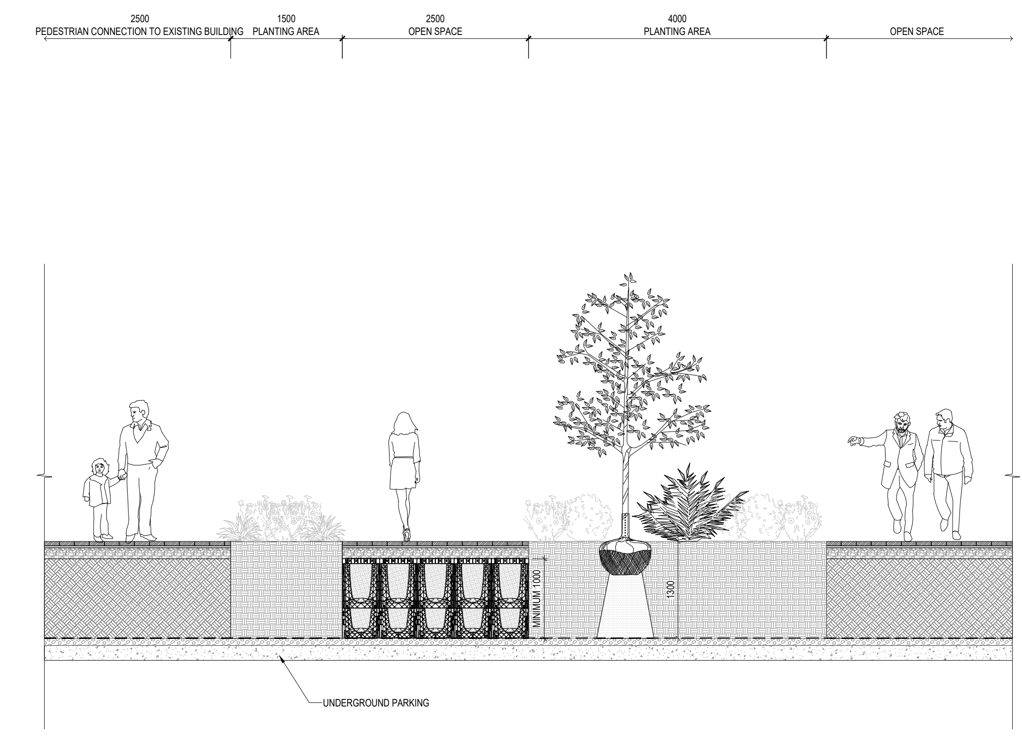
3 LANDSCAPE SECTION 3 OPEN SPACE 1:50
