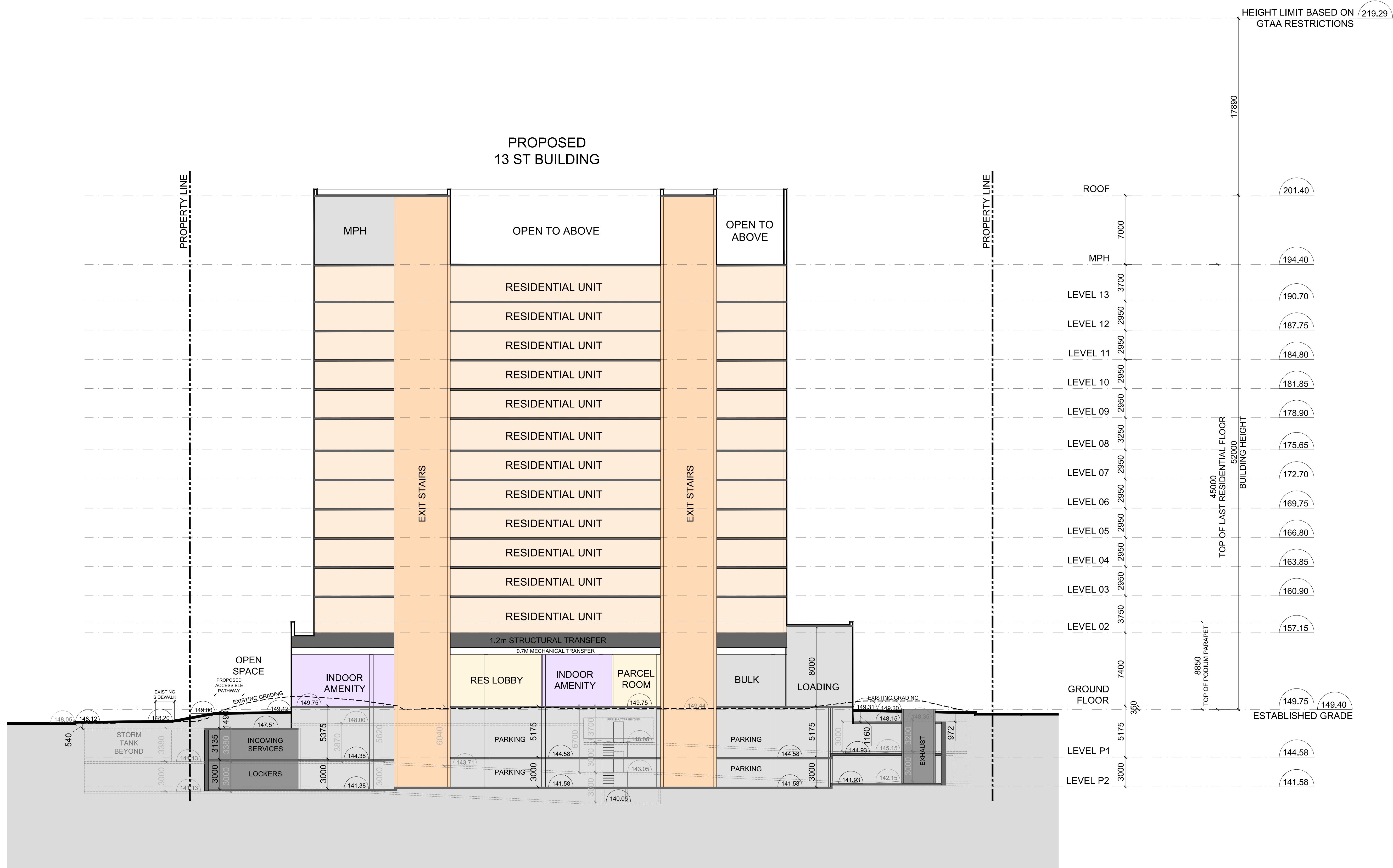
NORTH - SOUTH SECTION
