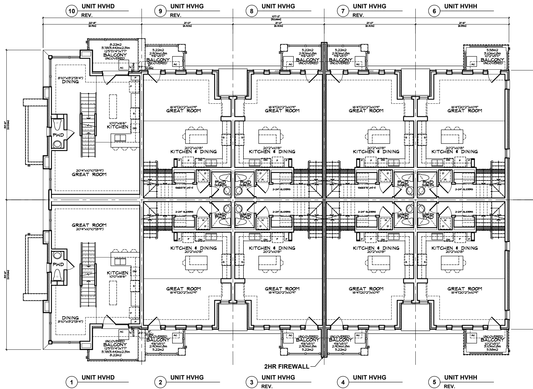
MAIN FLOOR PLAN 'MO' VILLAGE HOMES BLOCK 40
