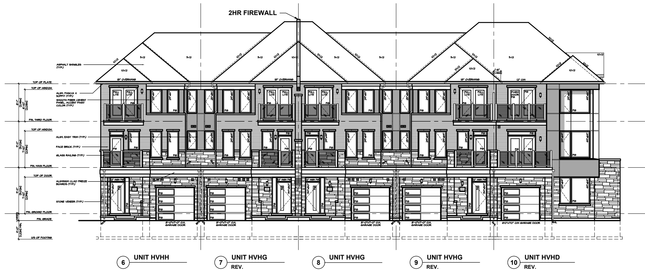
NORTH ELEVATION 'MO' VILLAGE HOMES BLOCK 40
