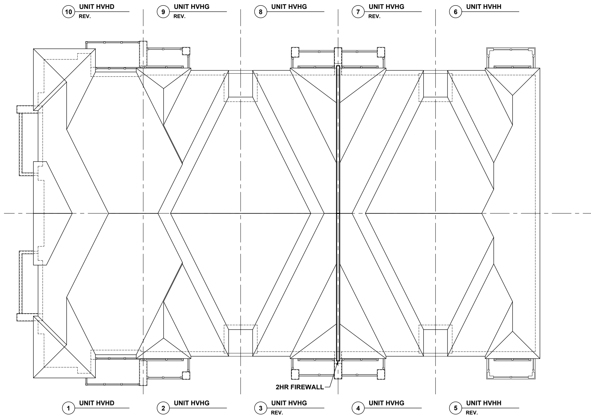
ROOF PLAN 'MO' VILLAGE HOMES BLOCK 40
