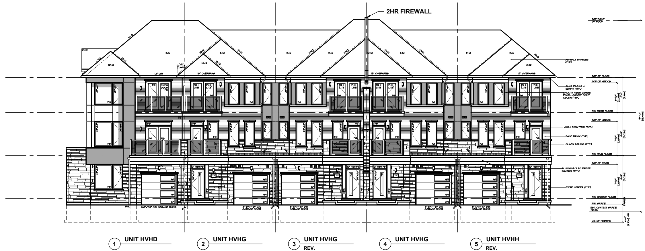
SOUTH ELEVATION 'MO' VILLAGE HOMES BLOCK 40
