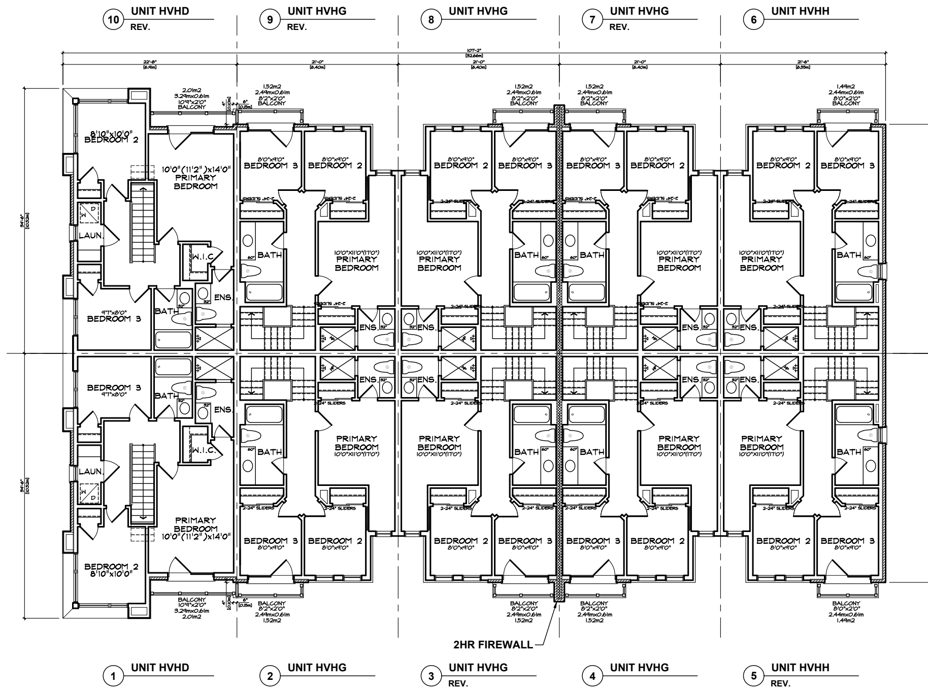
THIRD FLOOR PLAN 'MO' VILLAGE HOMES BLOCK 40
