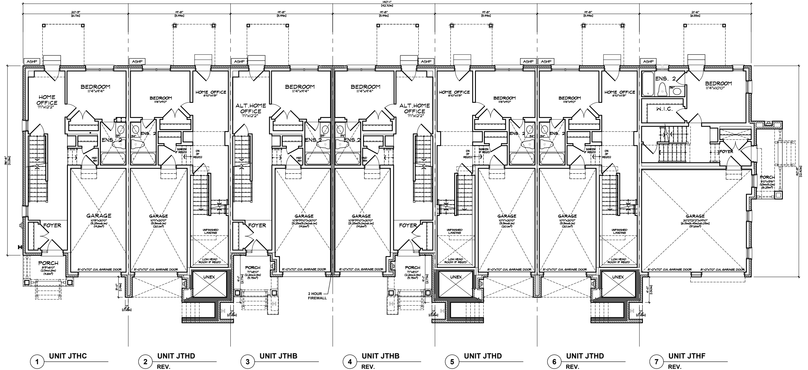
GROUND FLOOR PLAN 'MO' FRONTLOAD TOWNS BLOCK 32
