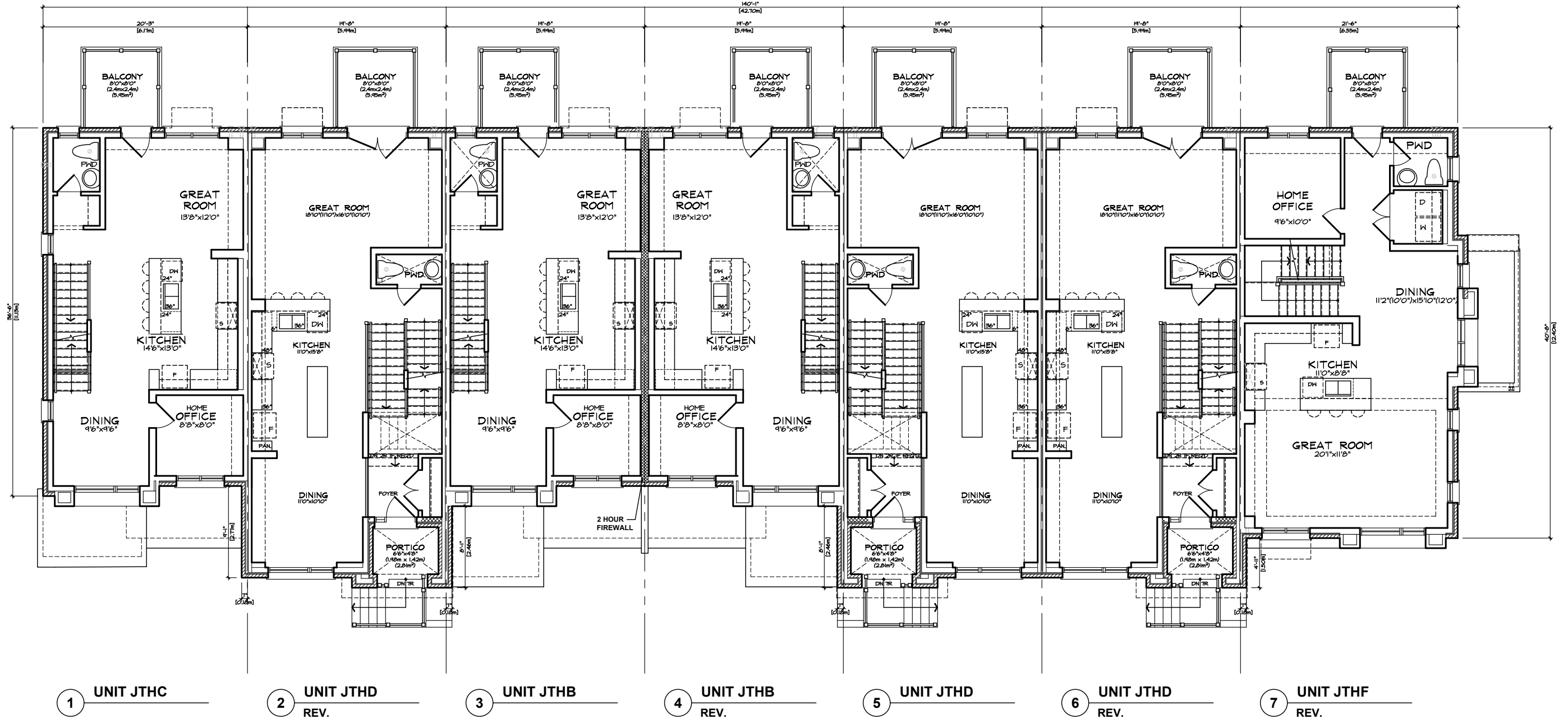
MAIN FLOOR PLAN 'MO' FRONTLOAD TOWNS BLOCK 32
