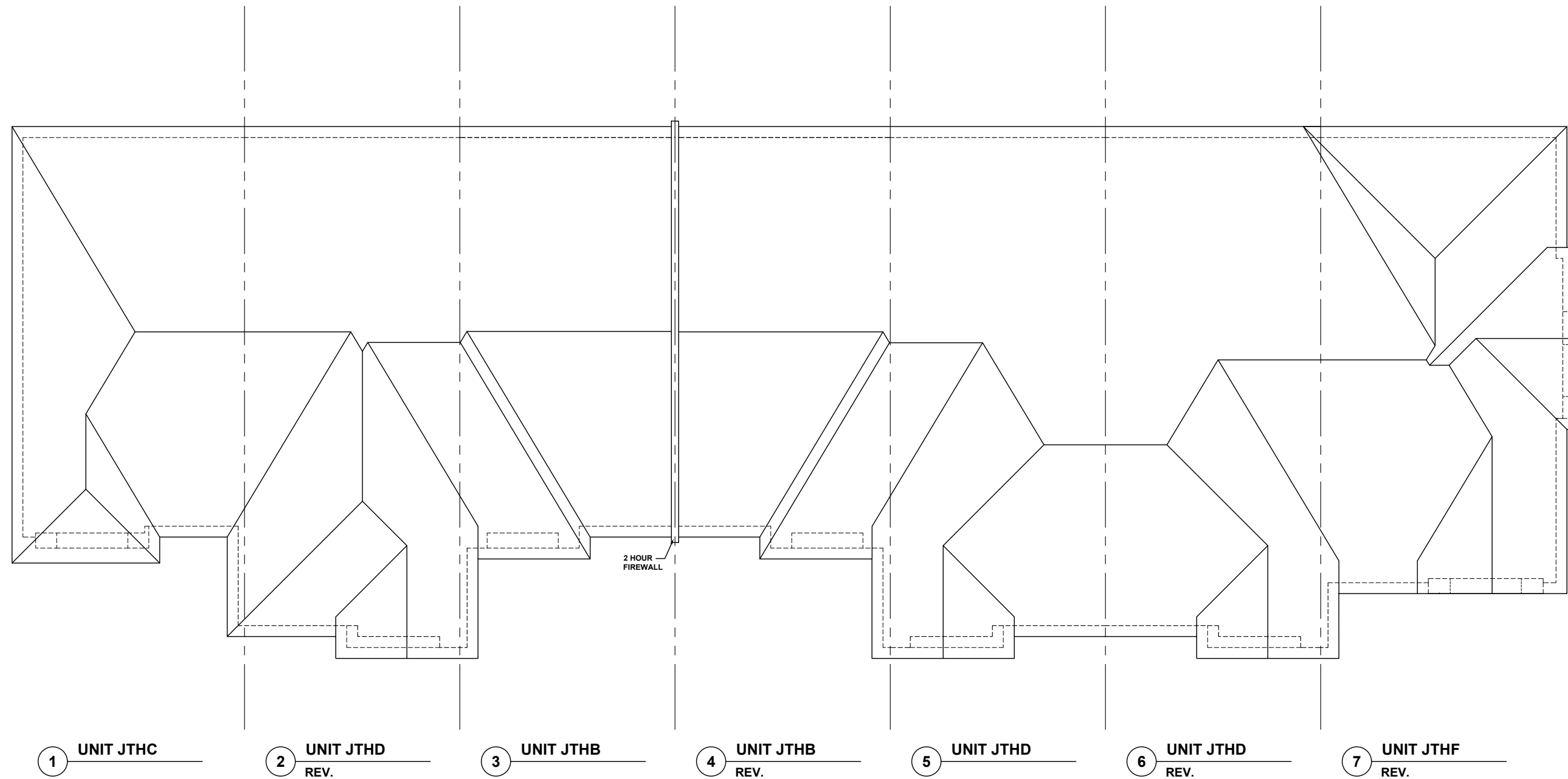
ROOF PLAN 'MO' FRONTLOAD TOWNS BLOCK 32
