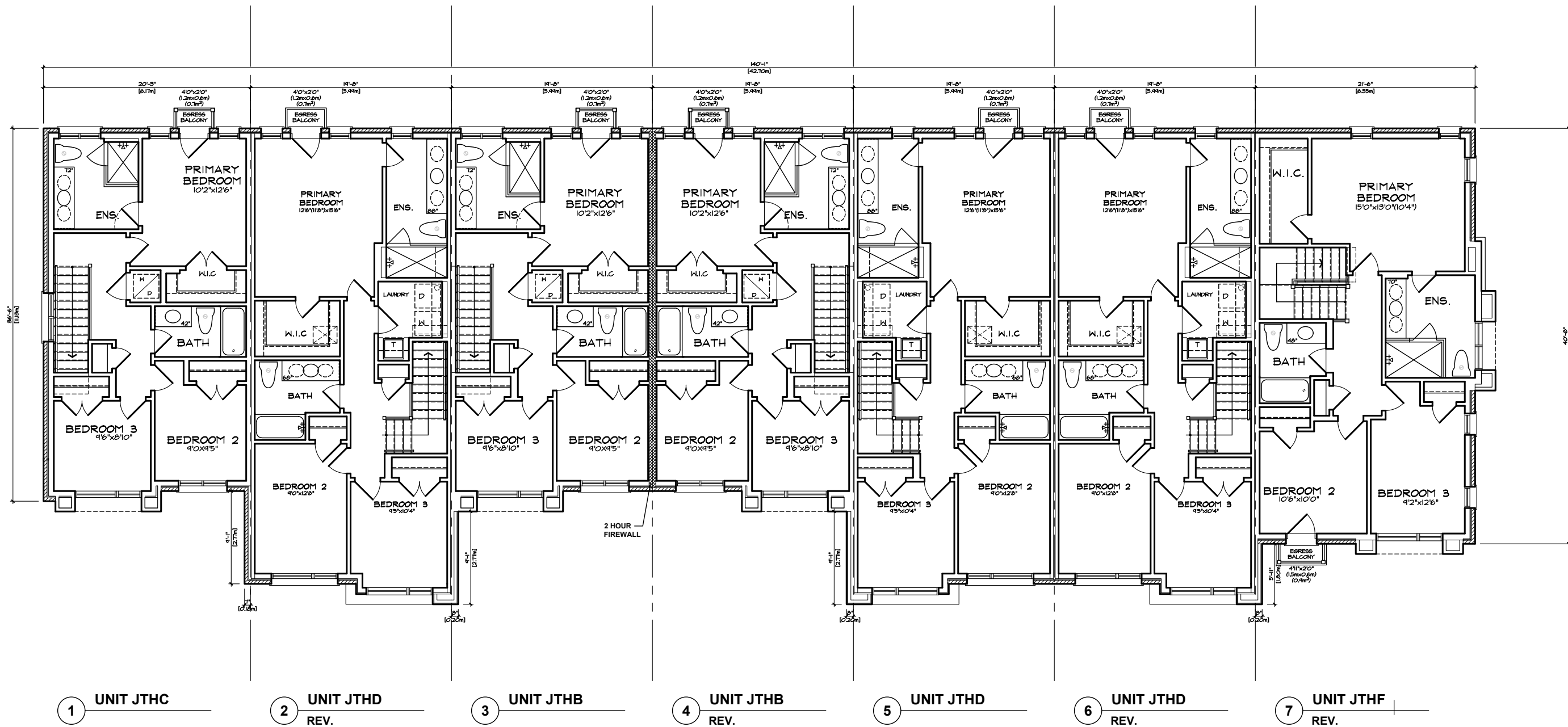
THIRD FLOOR PLAN 'MO' FRONTLOAD TOWNS BLOCK 32
