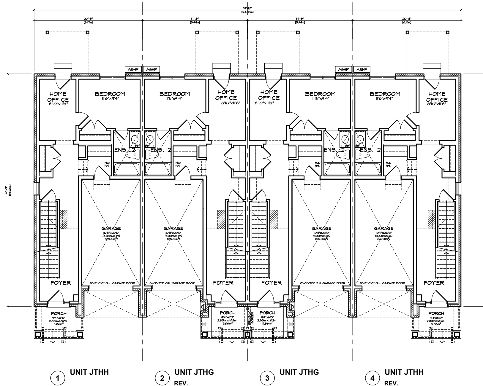
GROUND FLOOR PLAN 'FM' FRONTLOAD TOWNS BLOCK 33
