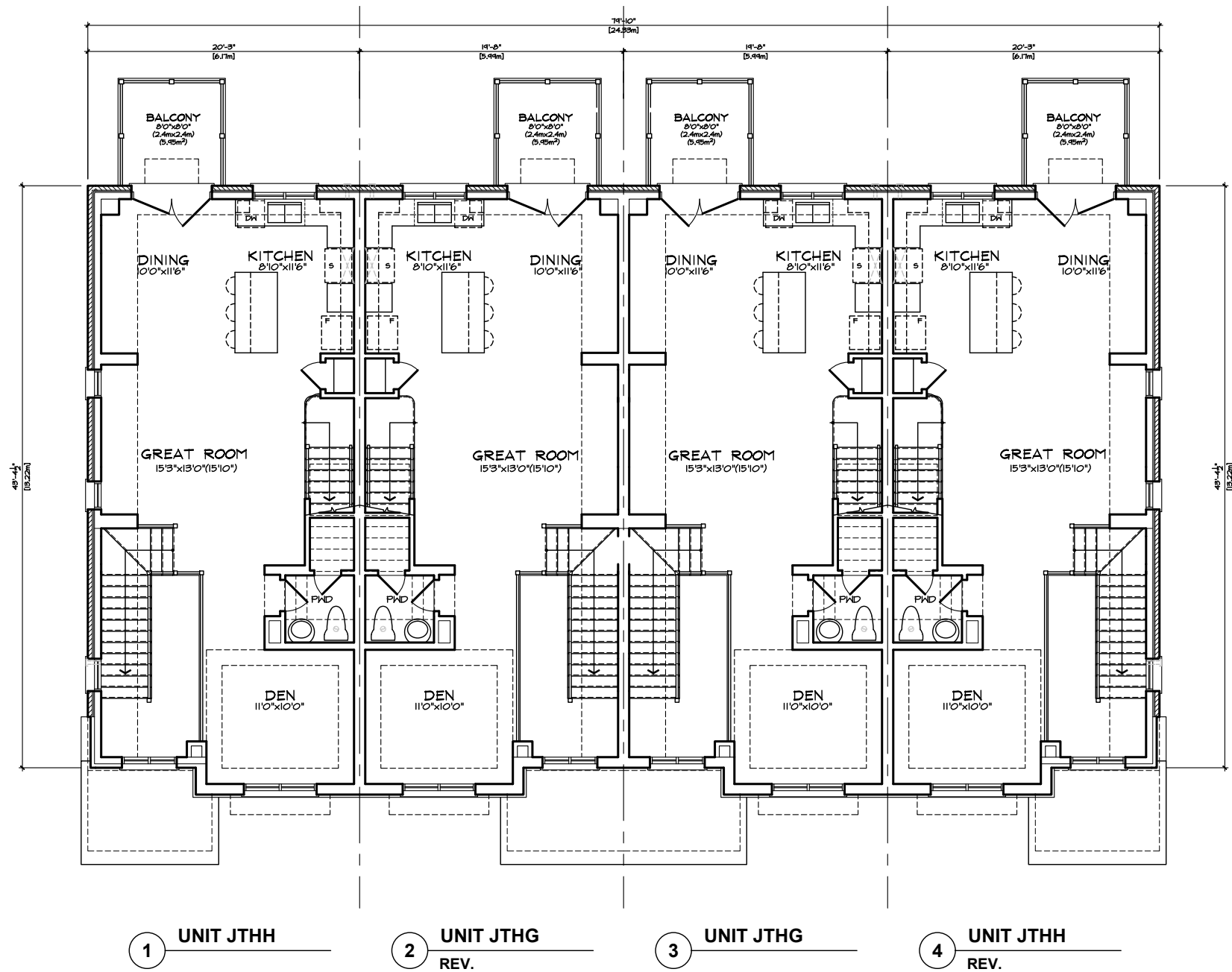
MAIN FLOOR PLAN 'FM' FRONTLOAD TOWNS BLOCK 33
