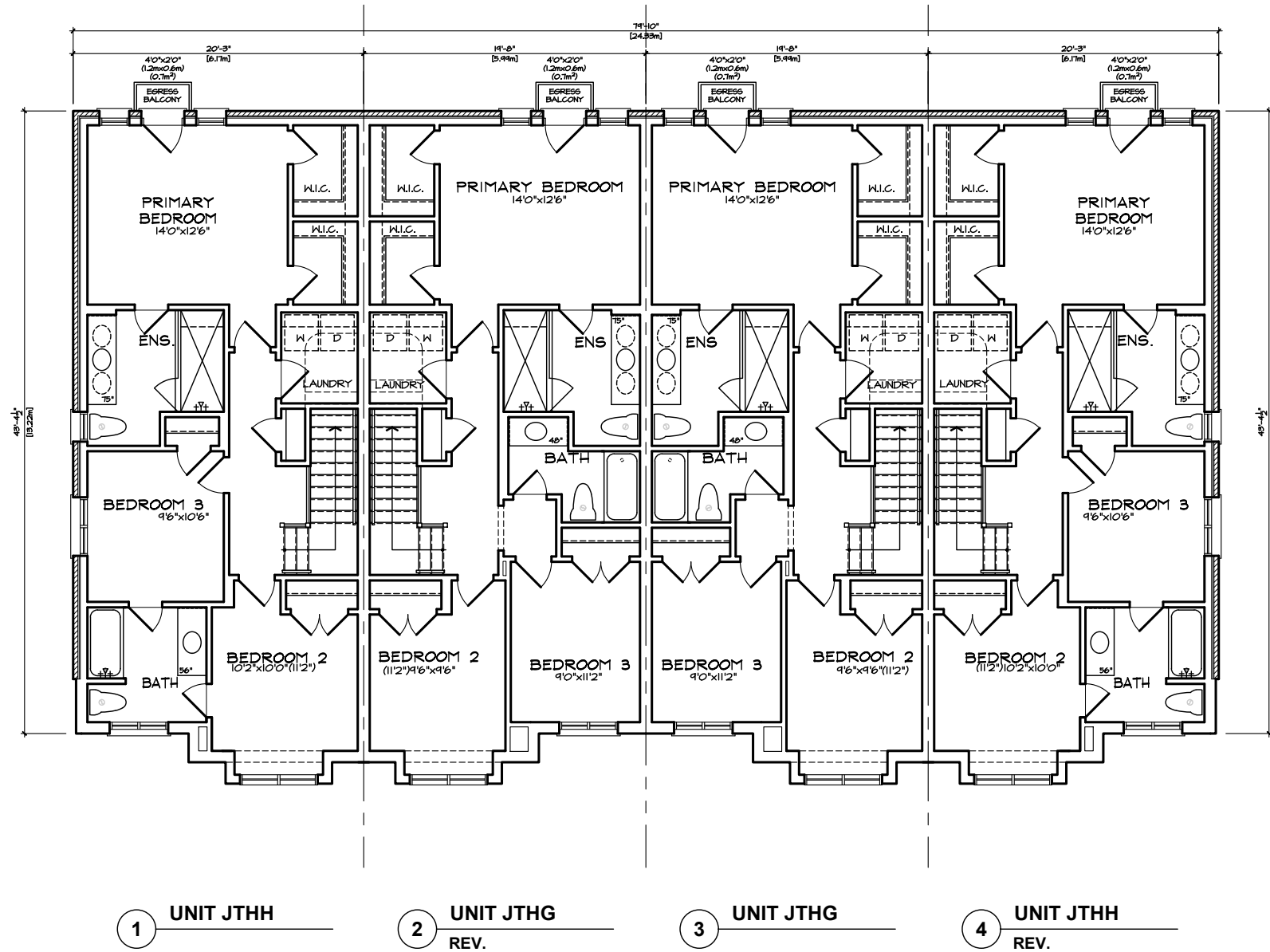
THIRD FLOOR PLAN 'FM' FRONTLOAD TOWNS BLOCK 33
