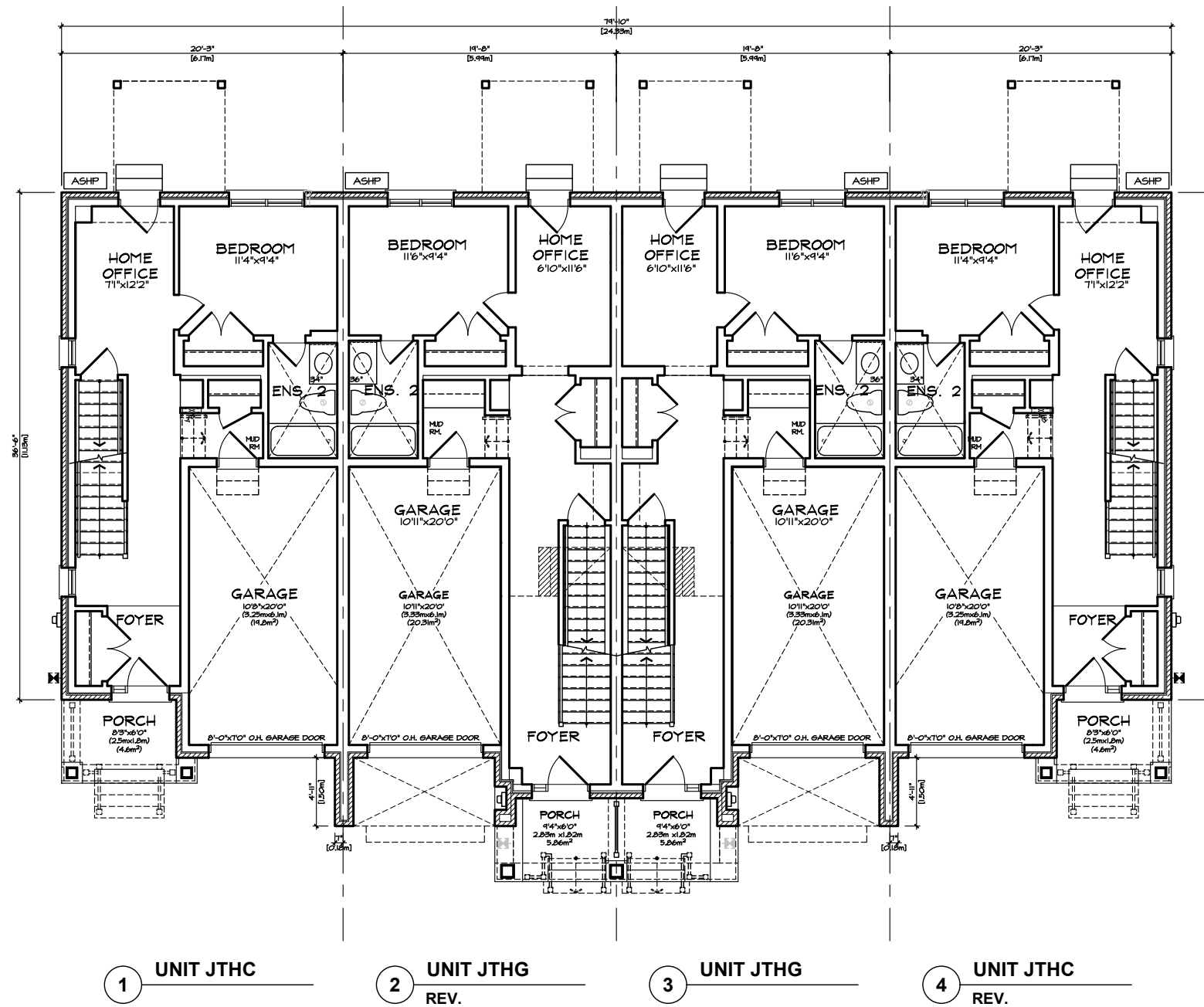
GROUND FLOOR PLAN 'FM' FRONTLOAD TOWNS BLOCK 34
