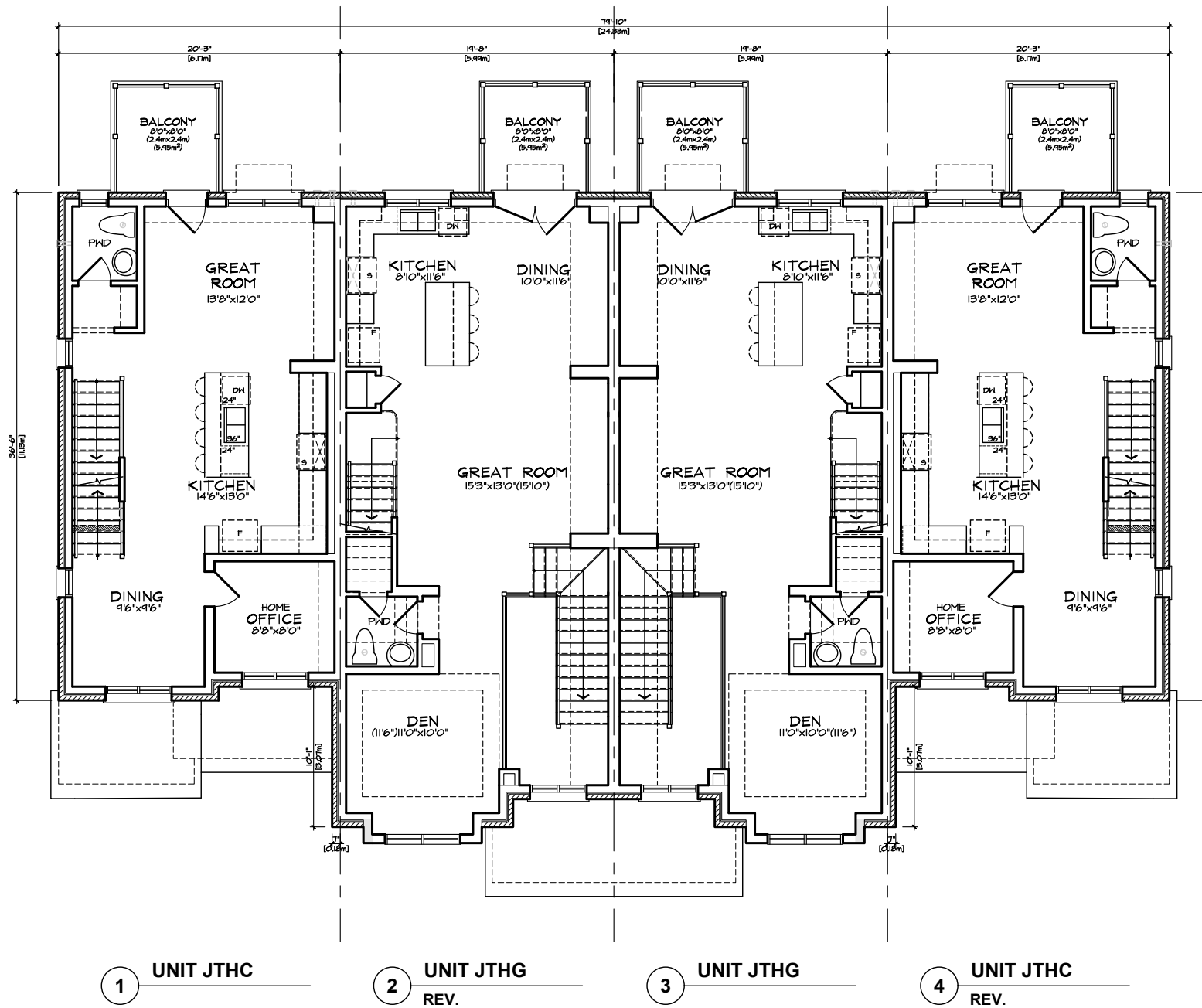
MAIN FLOOR PLAN 'FM' FRONTLOAD TOWNS BLOCK 34
