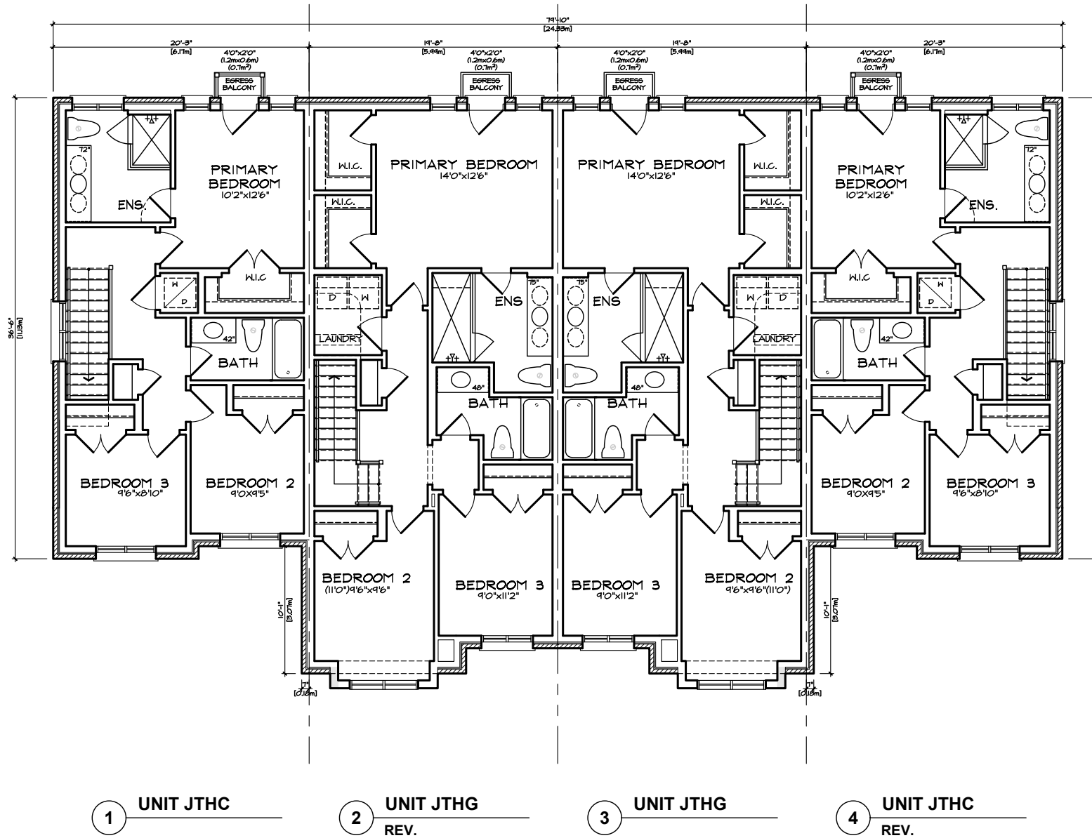
THIRD FLOOR PLAN 'FM' FRONTLOAD TOWNS BLOCK 34
