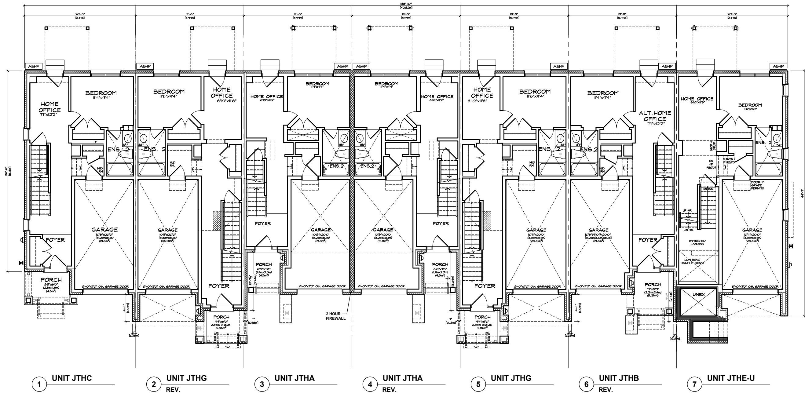
GROUND FLOOR PLAN 'MO' FRONTLOAD TOWNS BLOCK 35
