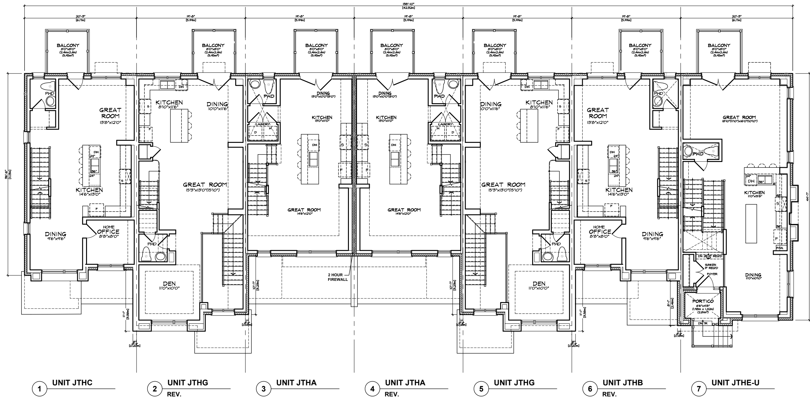
MAIN FLOOR PLAN 'MO' FRONTLOAD TOWNS BLOCK 35
