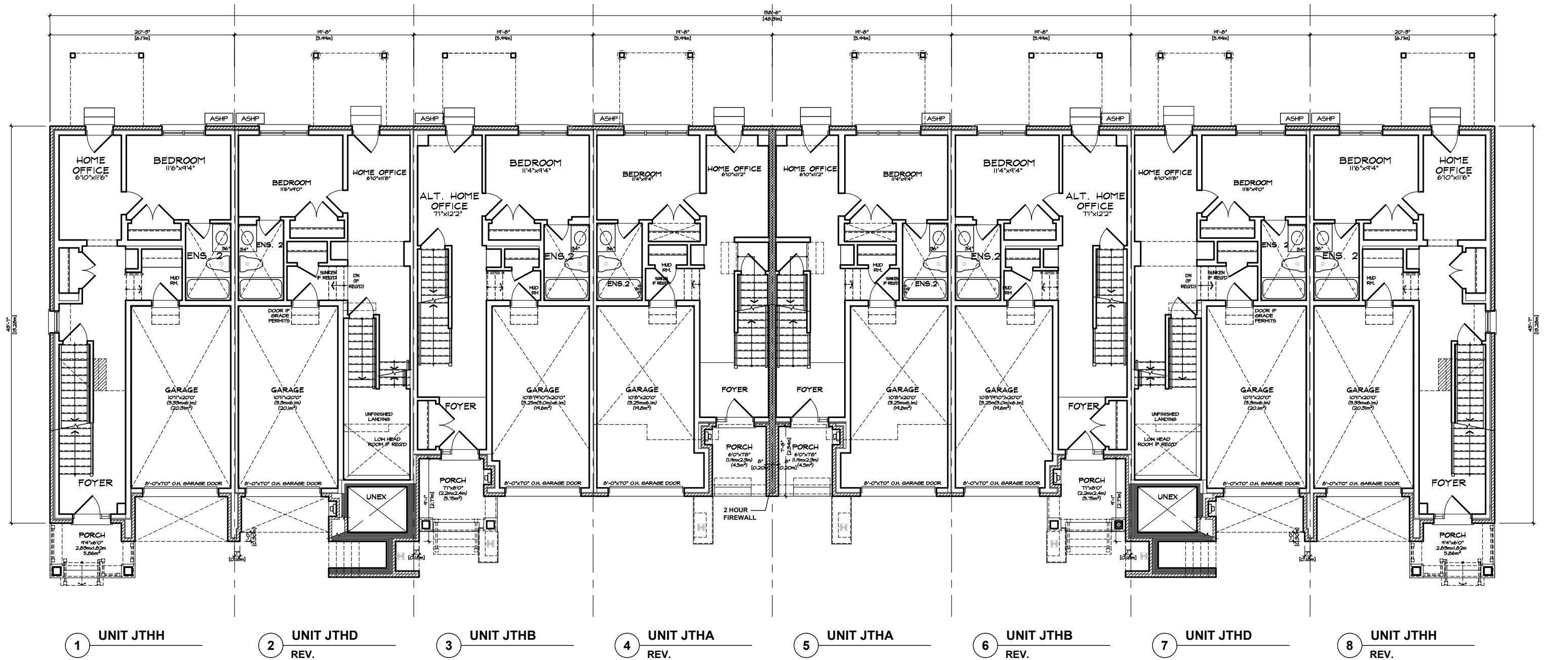
GROUND FLOOR PLAN 'FM' FRONTLOAD TOWNS BLOCK 36
