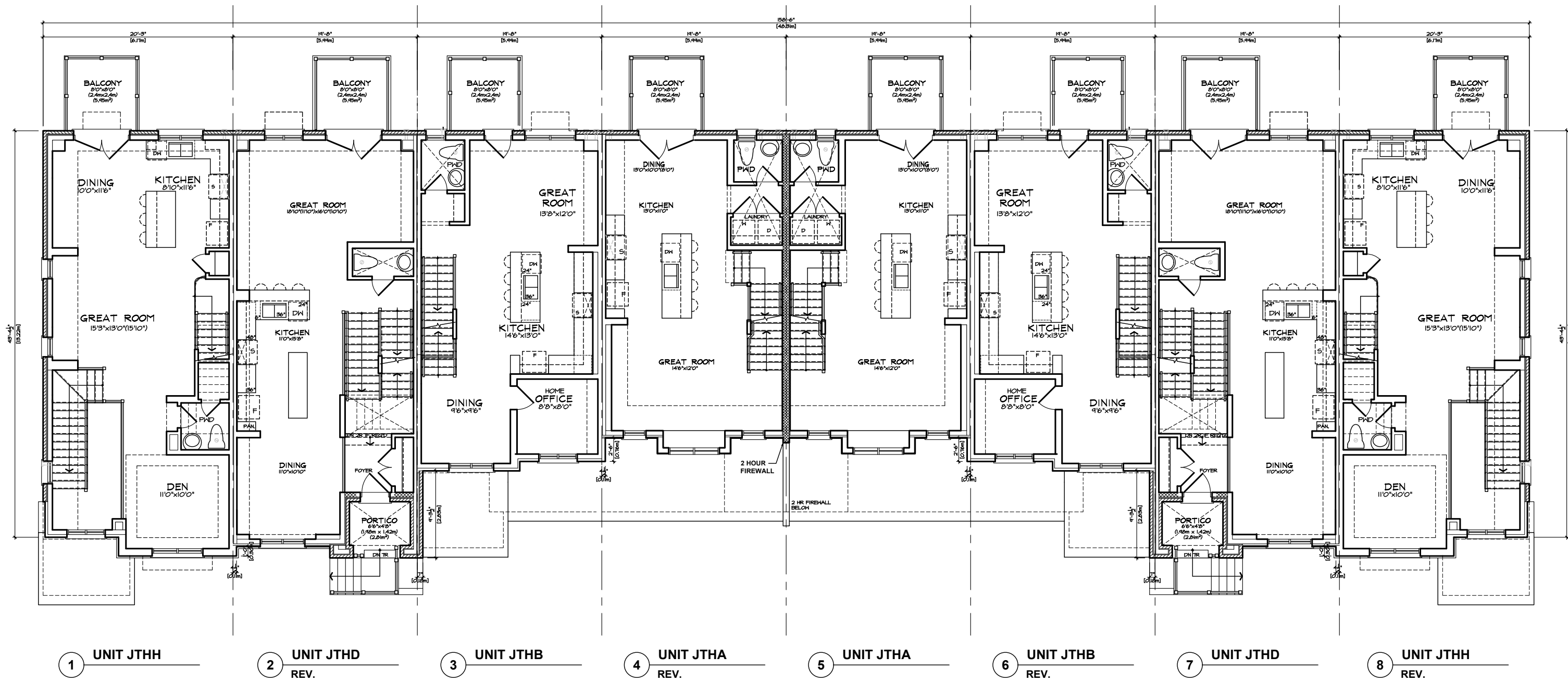
MAIN FLOOR PLAN 'FM' FRONTLOAD TOWNS BLOCK 36
