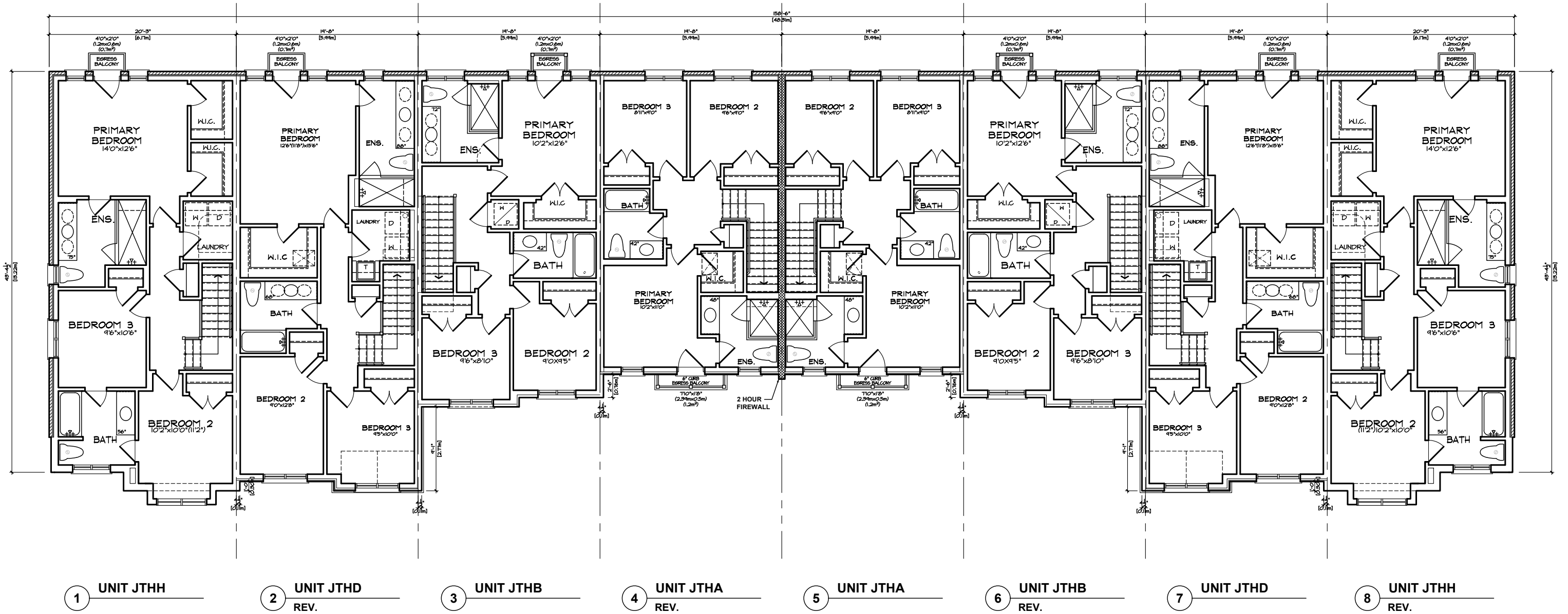
THIRD FLOOR PLAN 'FM' FRONTLOAD TOWNS BLOCK 36
